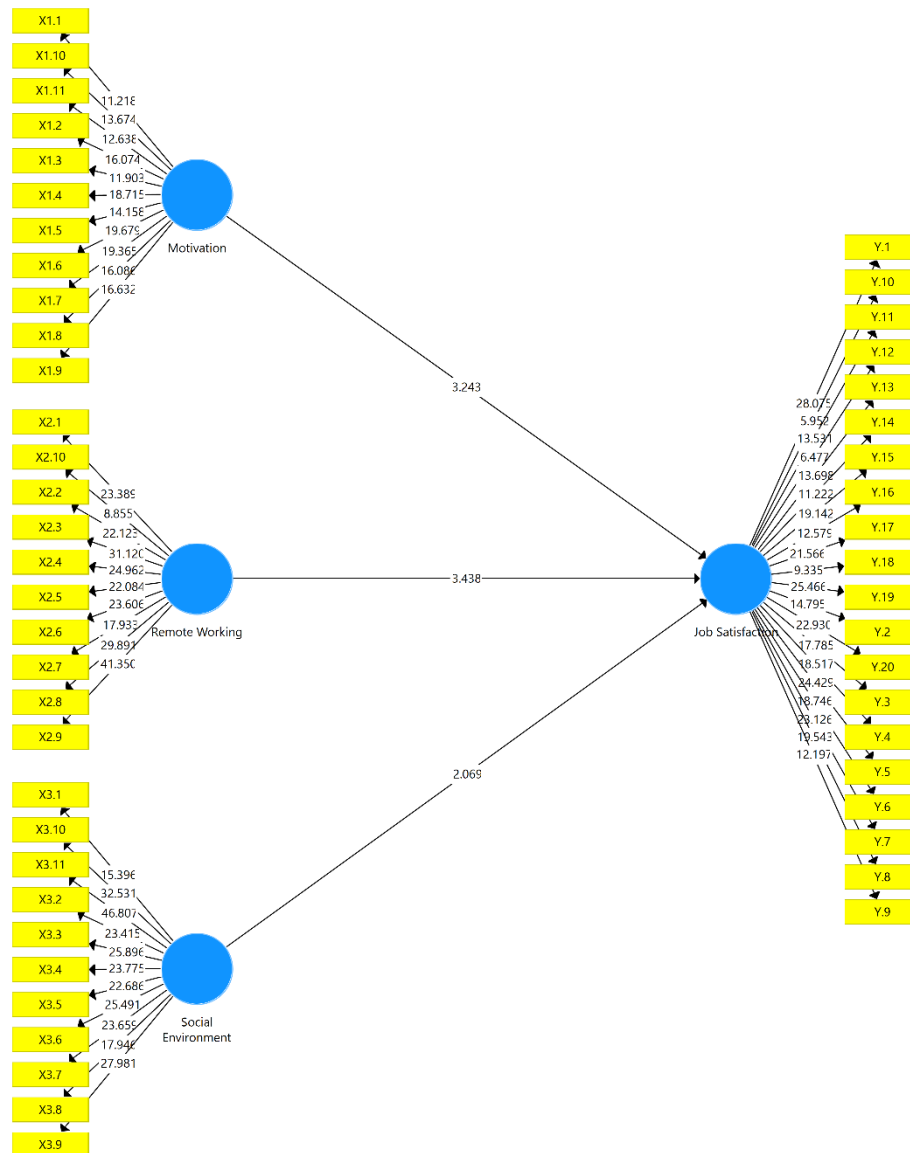
Fig. 2. Bootstrapping Results
