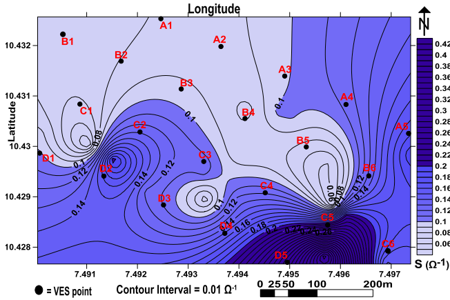
Fig 7: Longitudinal conductance of the area.
