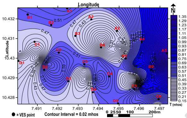
Fig 8: Protective Capacity of the study area.
