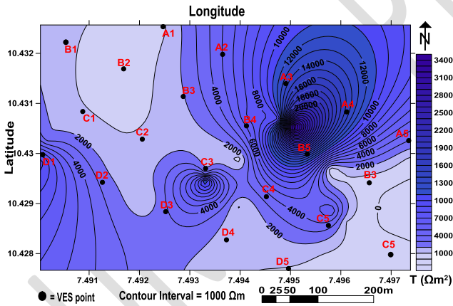
Fig 5: Transverse resistance of the study area.
