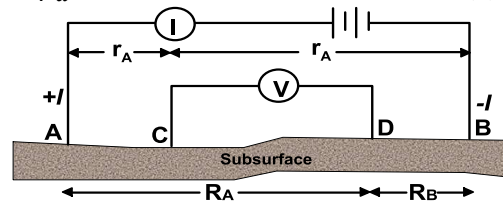
Fig. 2: Schlumberger Configuration
