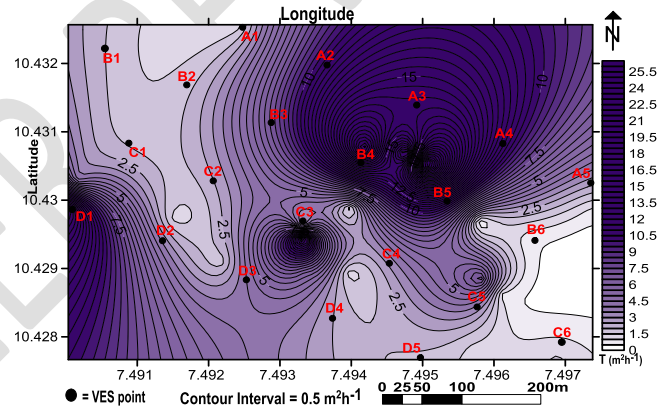
Fig 6: Transmissivity Map of the study area
