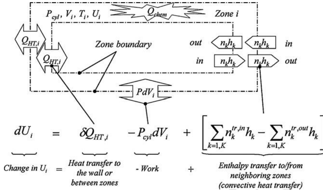
Fig. 5 : The First Law of Thermodynamics applied to a zone of a multi-zone model. (Komninos et Rakopoulos 2012)
