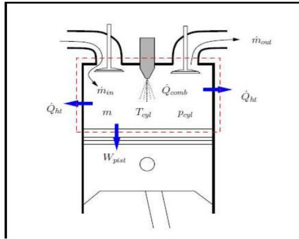
Fig 2: Heat balance of the single combustion zone model (Tarabet 2012)
