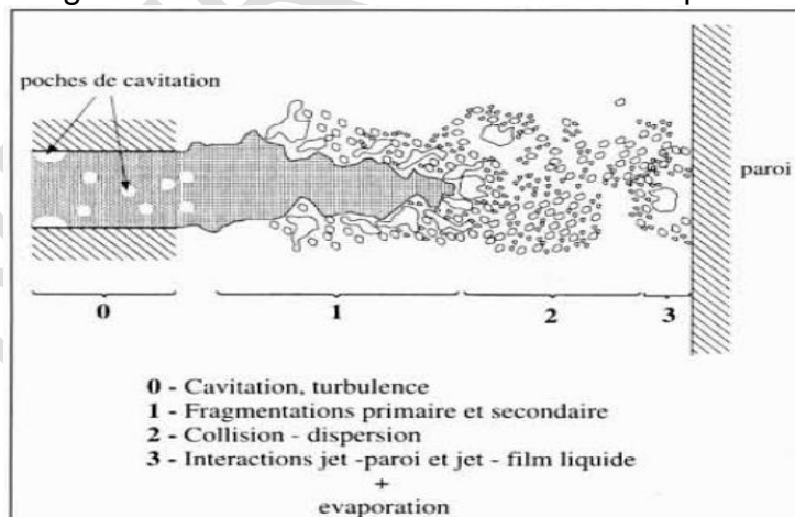
Fig 1: Schematic description of injection in a diesel engine (Mantel and Galzin 1998).
