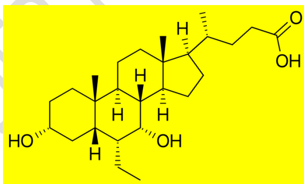
Fig 2: Obeticholic Acid
