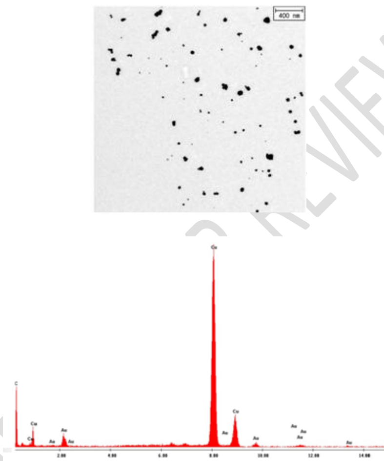
Figure-2: HR-TEM confirmation of crystallinity of the prepared Au nanoparticles and the mono-dispersion with EDAX spectrum confirm the purity
