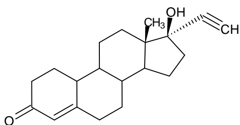
Figure 1: Norethindrone
