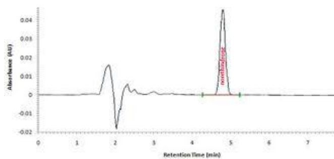
Figure 2: Chromatogram of norethindrone at concentration 0.5µg/ml in aqueous sample.
