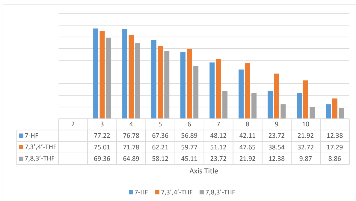
Fig. 1. In vitro MTT assay cytotoxicity effect of test substance 7-HF, 7,3',4'-THF and 7,8,3'-T
