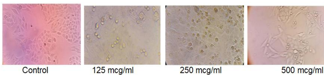
Fig 3. In vitro (MTT assay) cytotoxicity effect of test substance 7,3',4'THF against MCF-7 cell line
