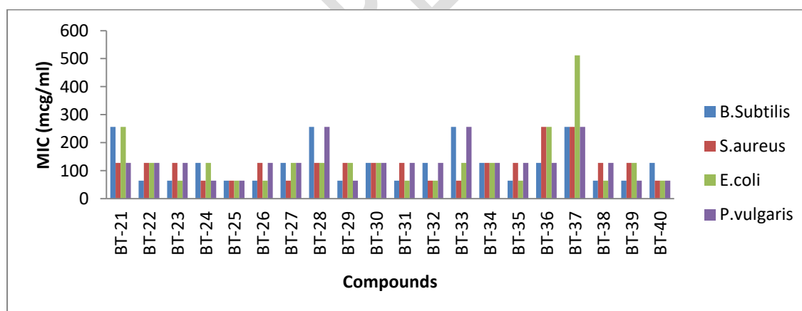
Figure 3: Antibacterial activity of Benzothiazepines (BT-21to BT-40): (Expressed as MIC in \mu\text{g/ml} )
