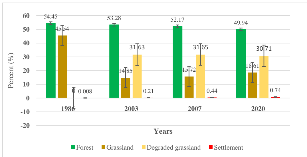
Figure 2: Percentage of Land use change statistics in Ajei Area
