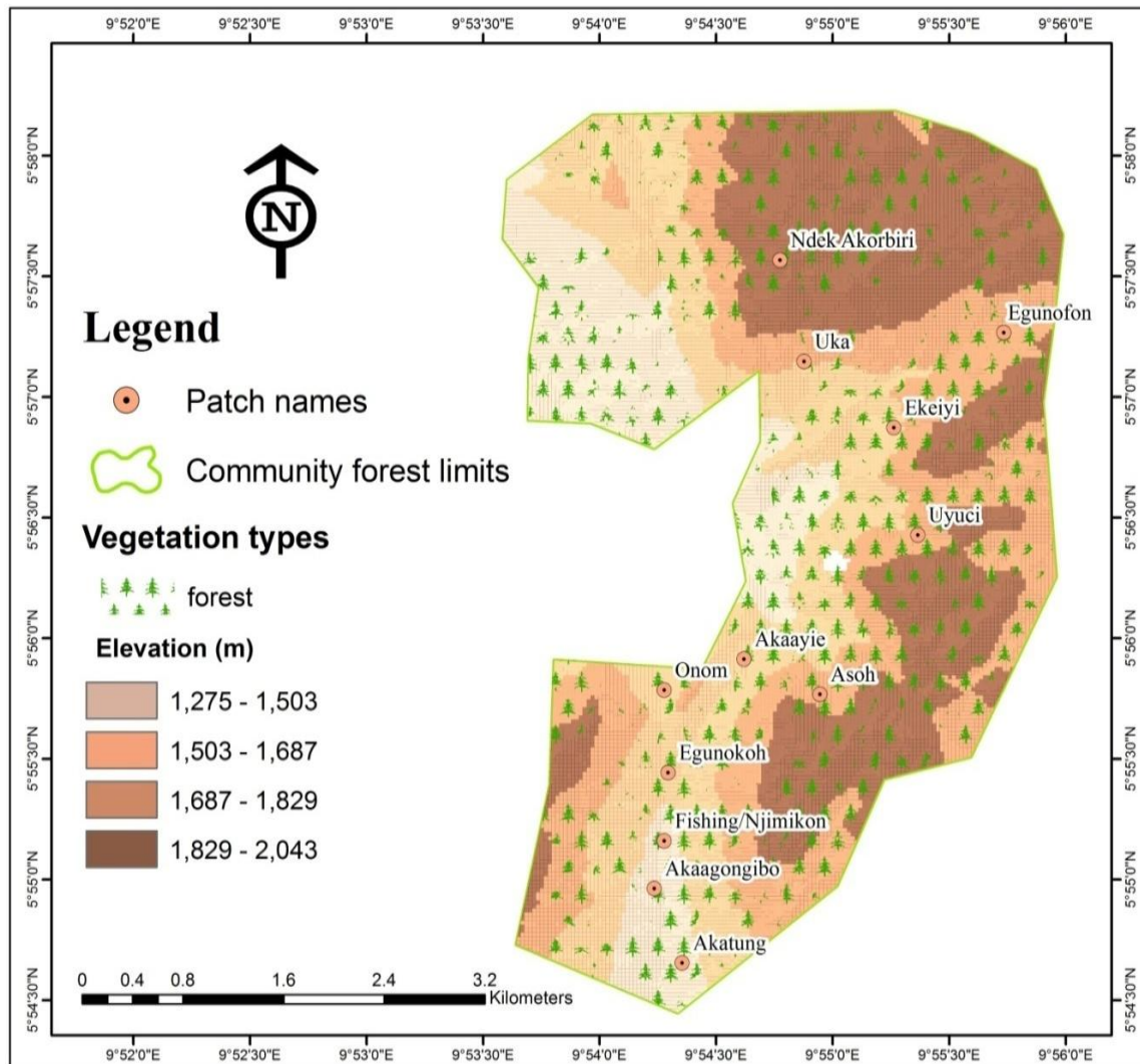
Figure 7: Relief and Vegetation features in the Ajei Area
