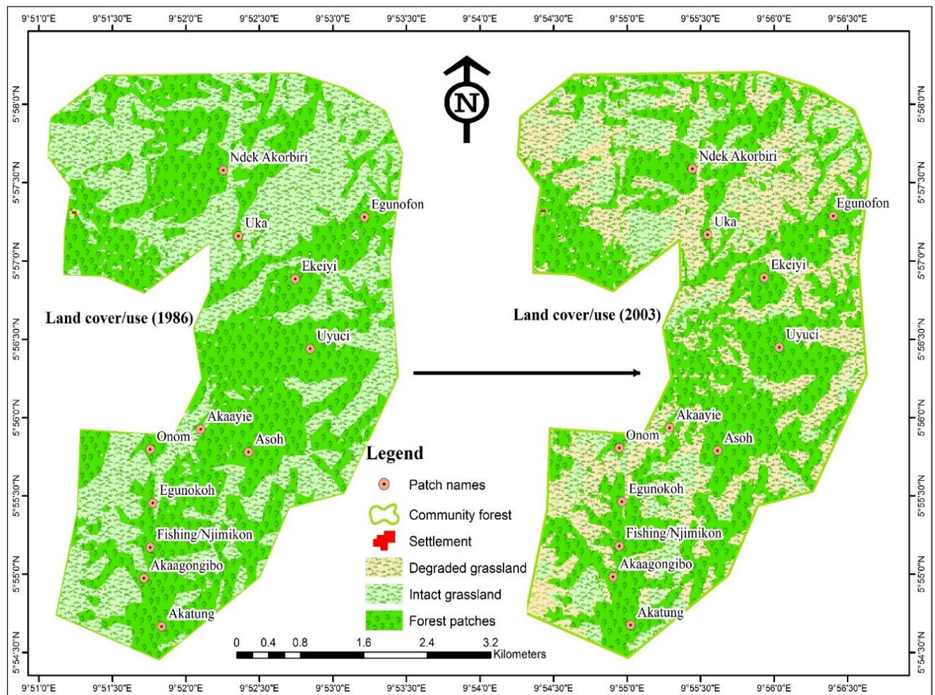
Figure 3: Land use for 1986 and 2003 Source: Classified Landsat, (1986) and ASTER, (2003)
