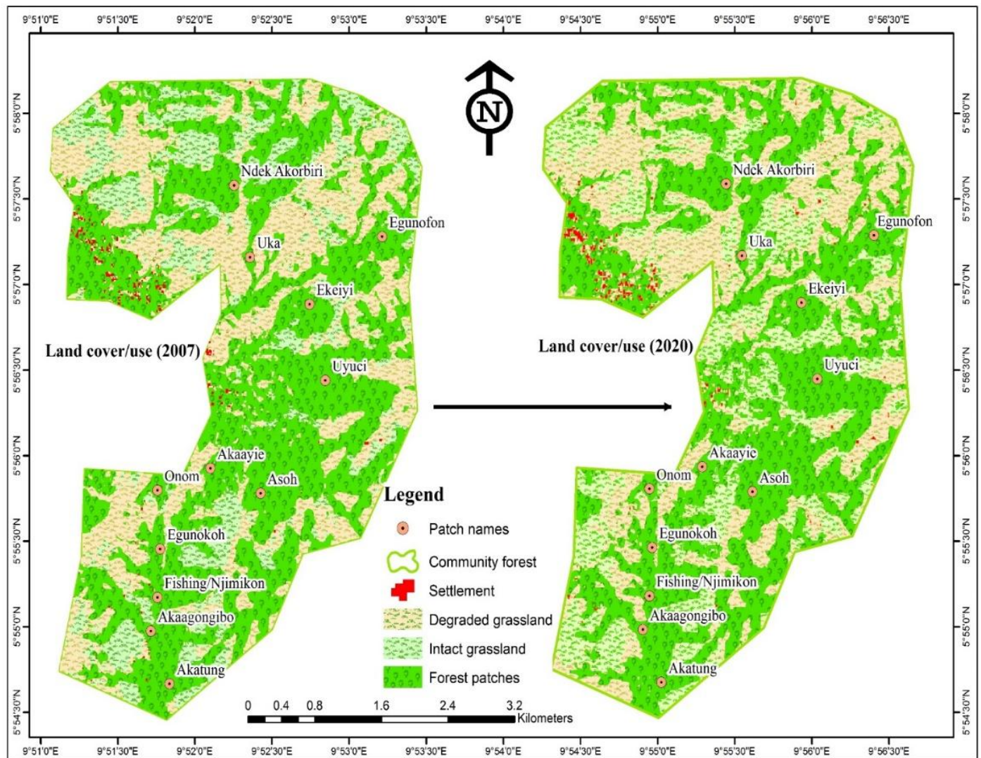
Figure 4: Land use for 2007 and 2020 Source: Classified ASTER, (2007 and 2020)
