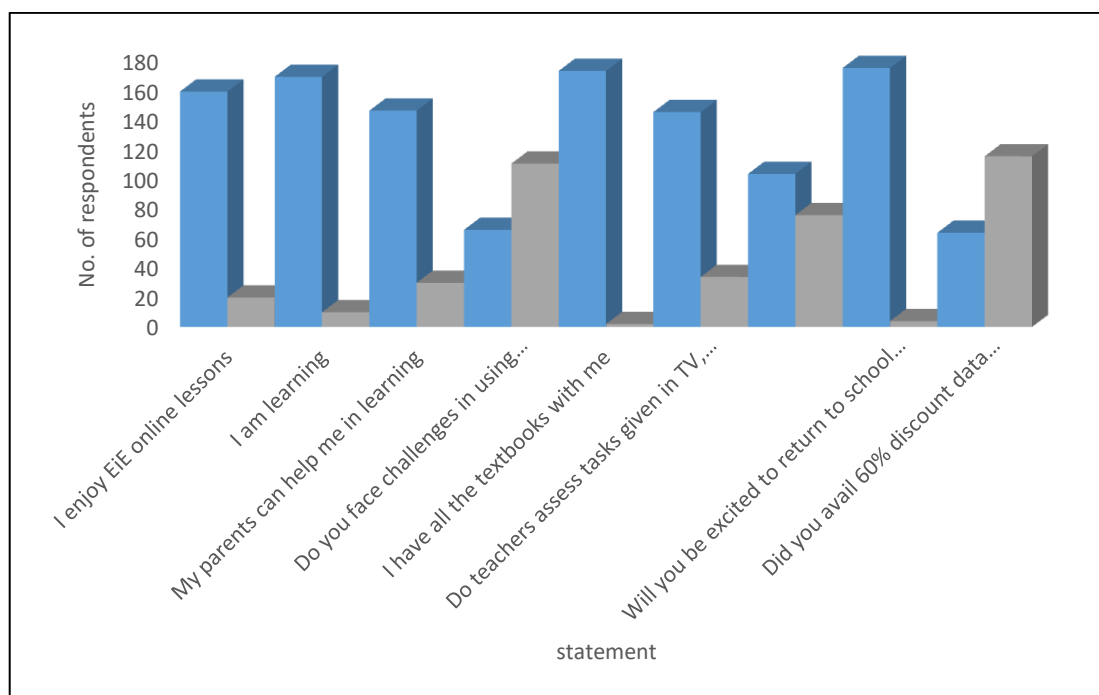
Figure 1: Categorical Variables
