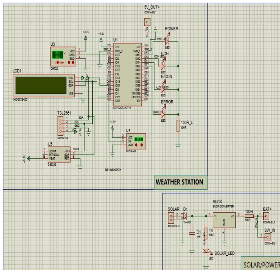
Fig. 6. Circuit diagram
