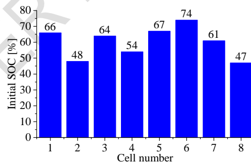
Fig.6.Initial SOC
