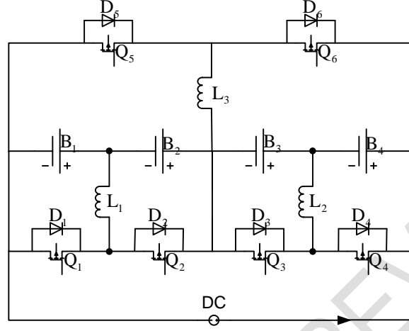
Fig.2. Battery pack equalization circuit
