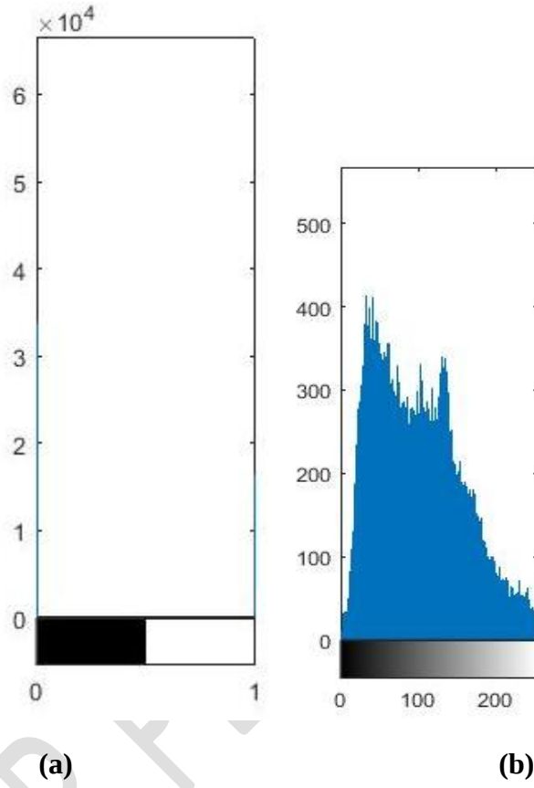
Fig.7a and b: Binary equivalence of sample image A and Histogram equivalence of sample image A
