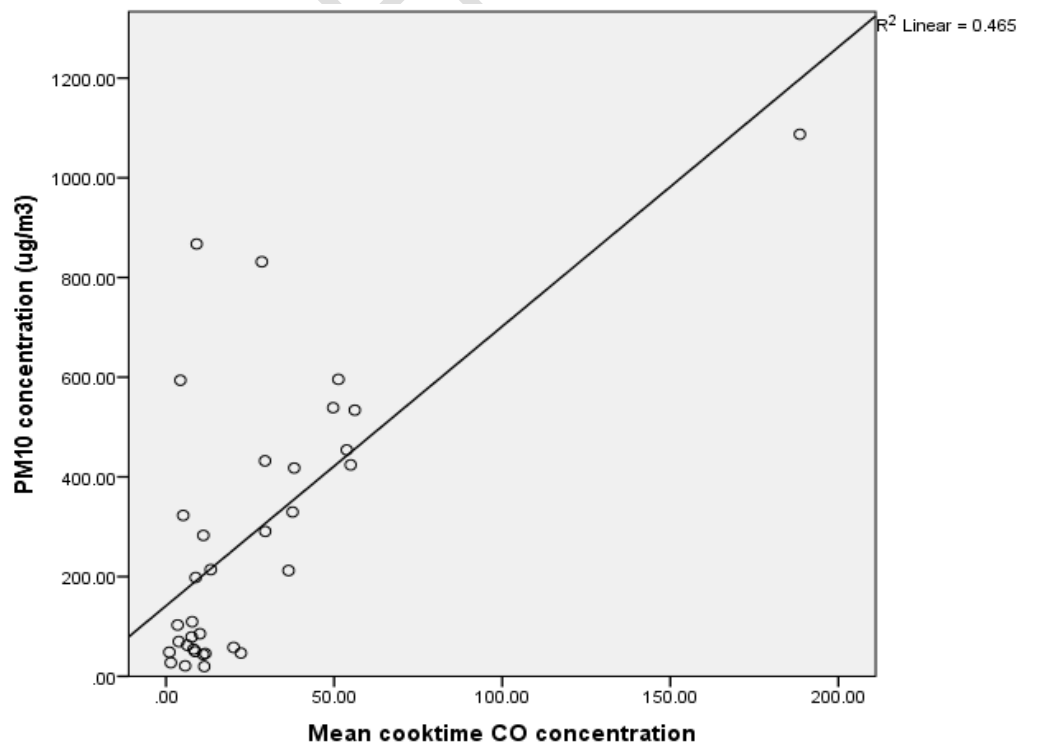
Figure 7: Scatter plot of Mean CO vs PM 10 concentrations
