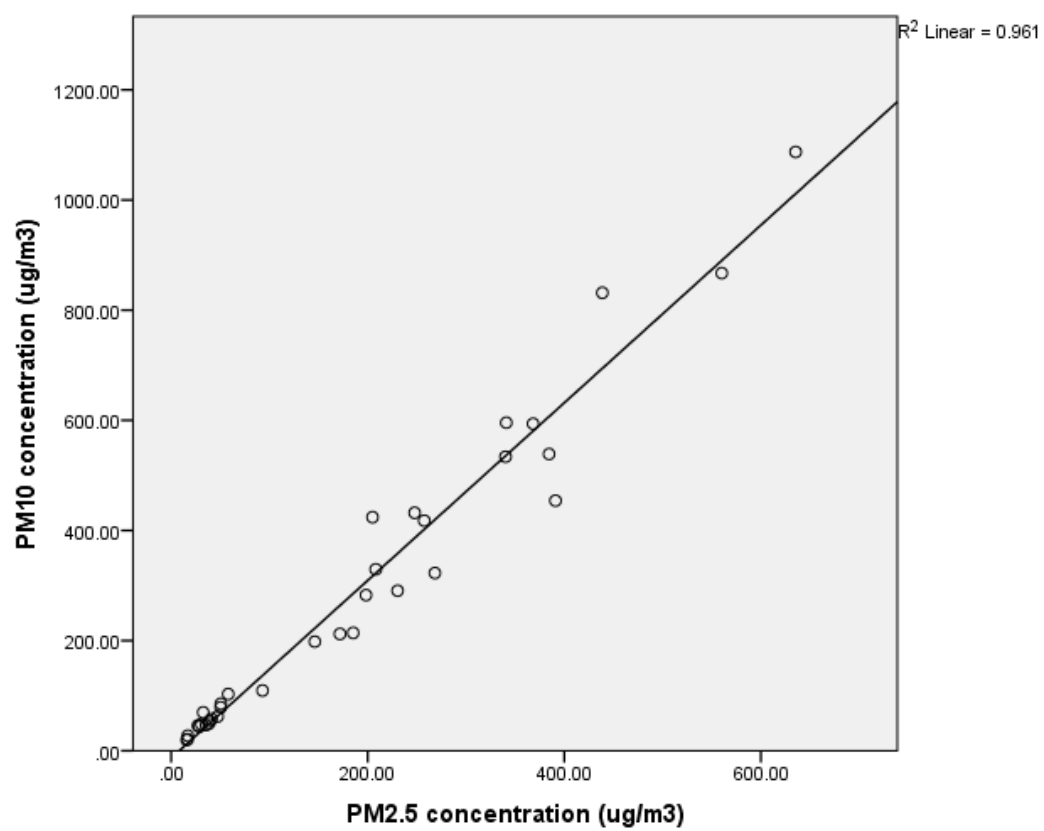
Figure 8: Scatter plot of Mean PM 10 vs PM 2.5 concentrations
