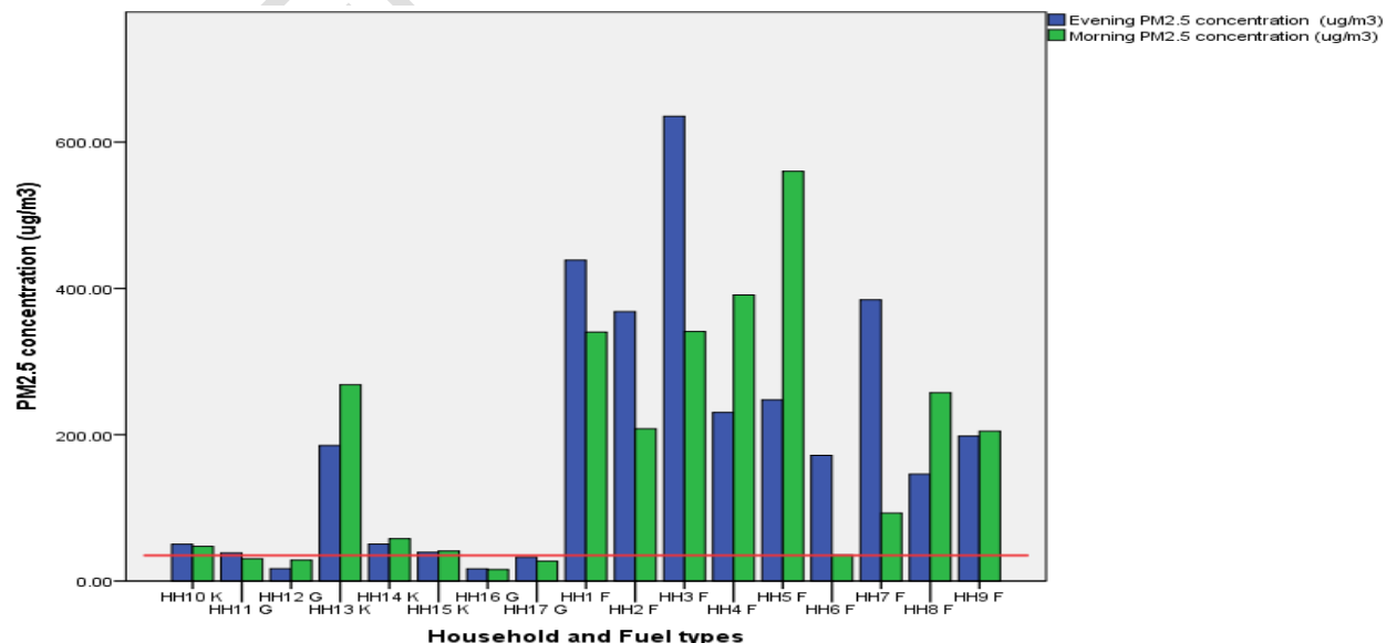
Figure 5: Comparison of 1-hr Mean morning and evening PM 2.5 concentration with WHO Interim-Target-1 recommendation.
