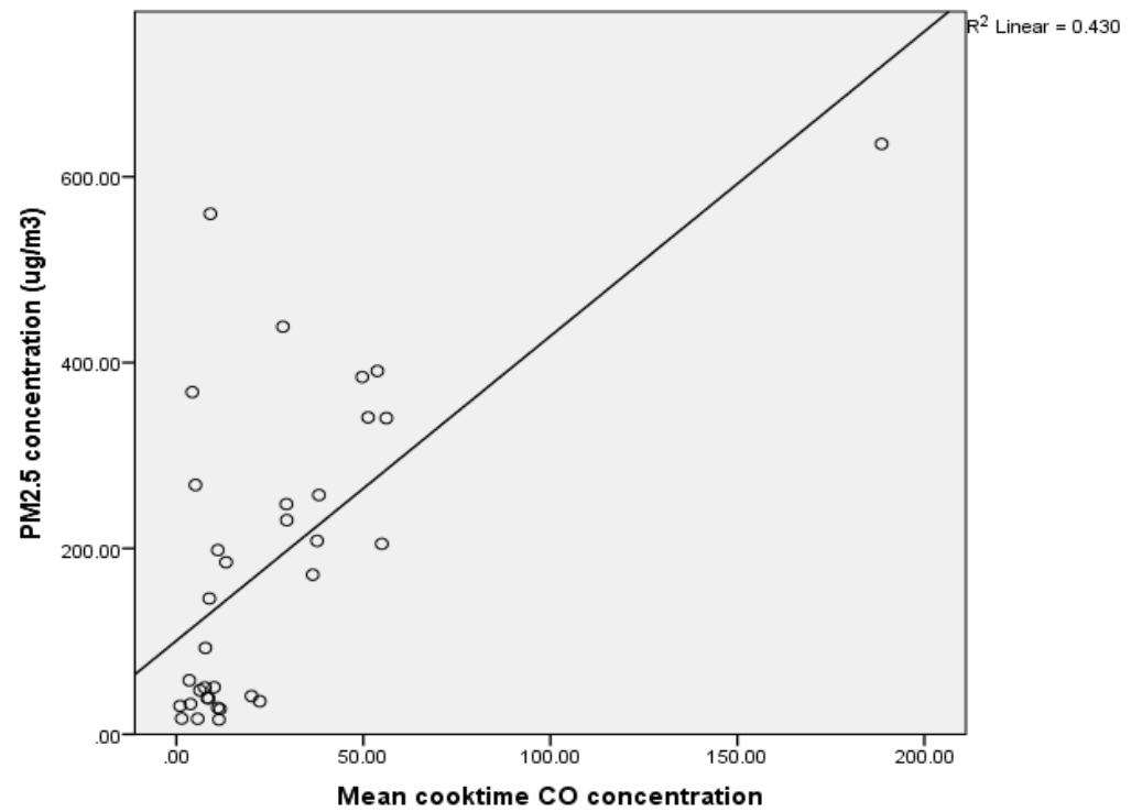
Figure 6: Scatter plot of Mean CO vs PM 2.5 concentrations
