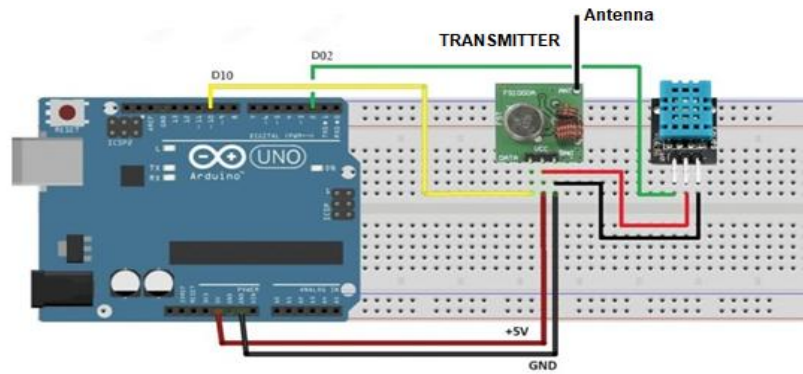
Figure 5. Transmission unit
