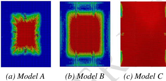
Fig.7 Plastic damage of the bottom of slab under ultimate load
