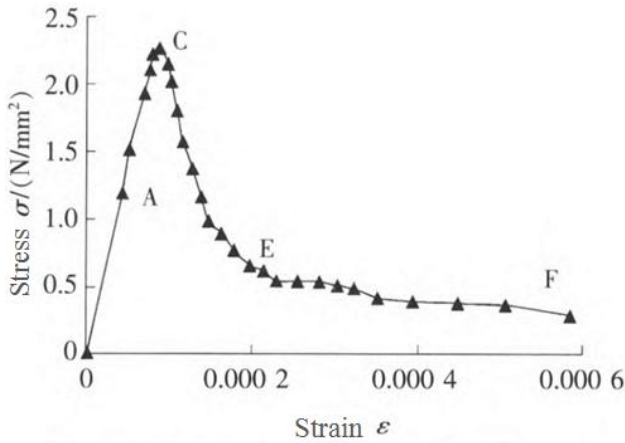
Fig.4 The Tensile stress-strain curve of concrete
