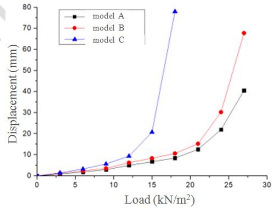
Fig.6 The midspan load-displacement curve of three kinds of slabs
