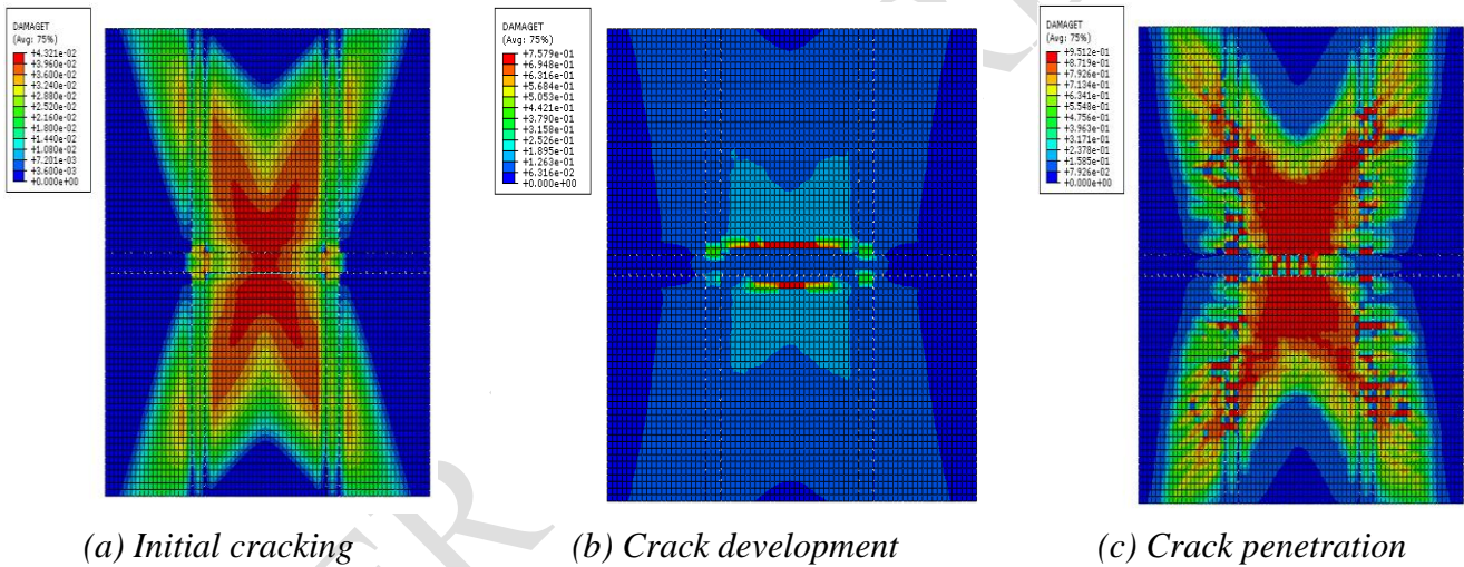
Fig.10 Damage distribution in different stress stages of model C
