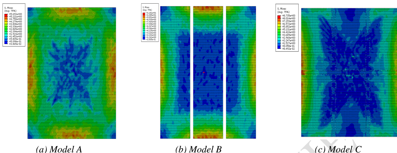
Fig.11 Stress distribution of three kinds of slabs in cracks penetration stage
