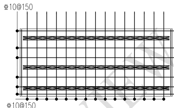
Fig.2 The rebar drawing of composite slab
