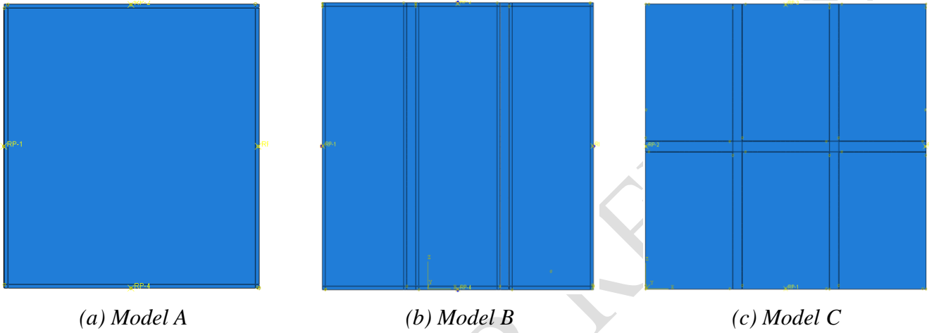
Fig.5 Schematic diagram of composite slab with different splicing methods
