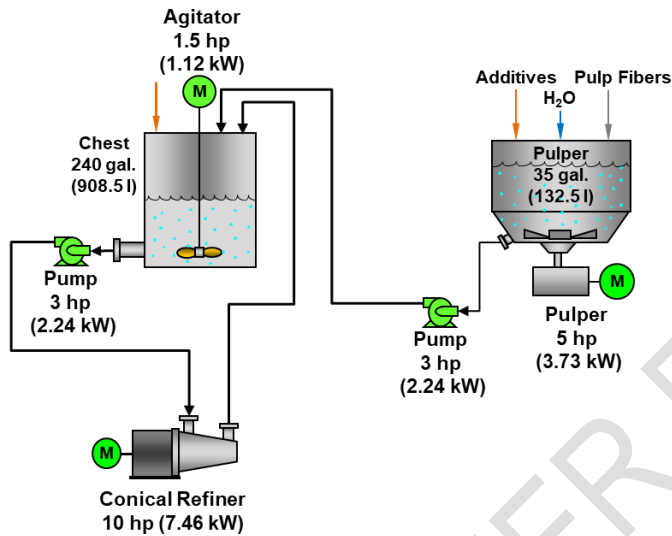
Fig. 2. Laboratory stock preparation system [40].
