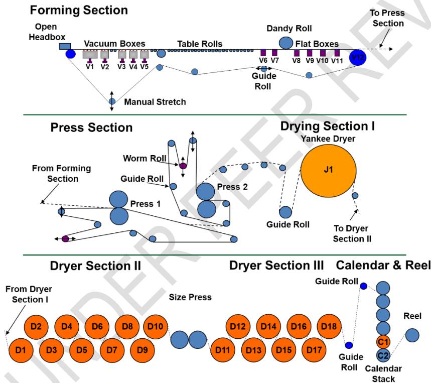
Fig. 4. Laboratory Fourdrinier paper machine [40].
