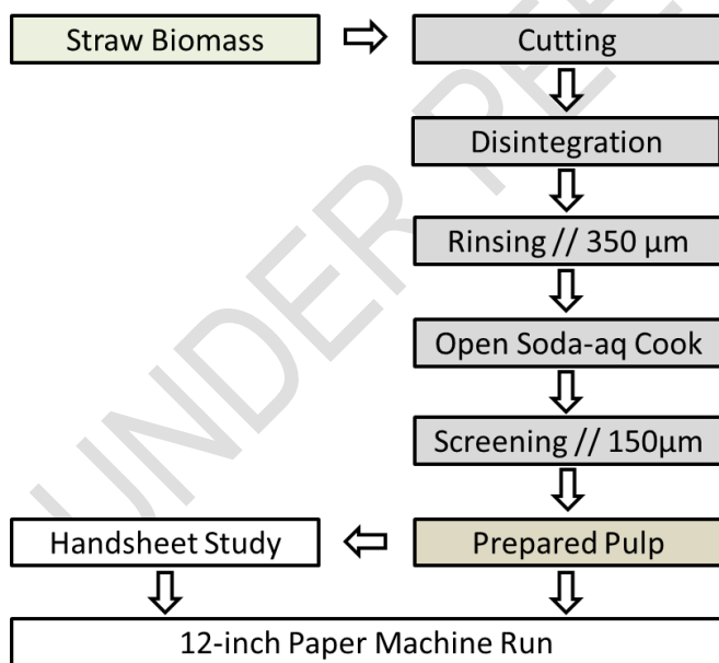
Fig. 1. Wheat straw processing flow chart
