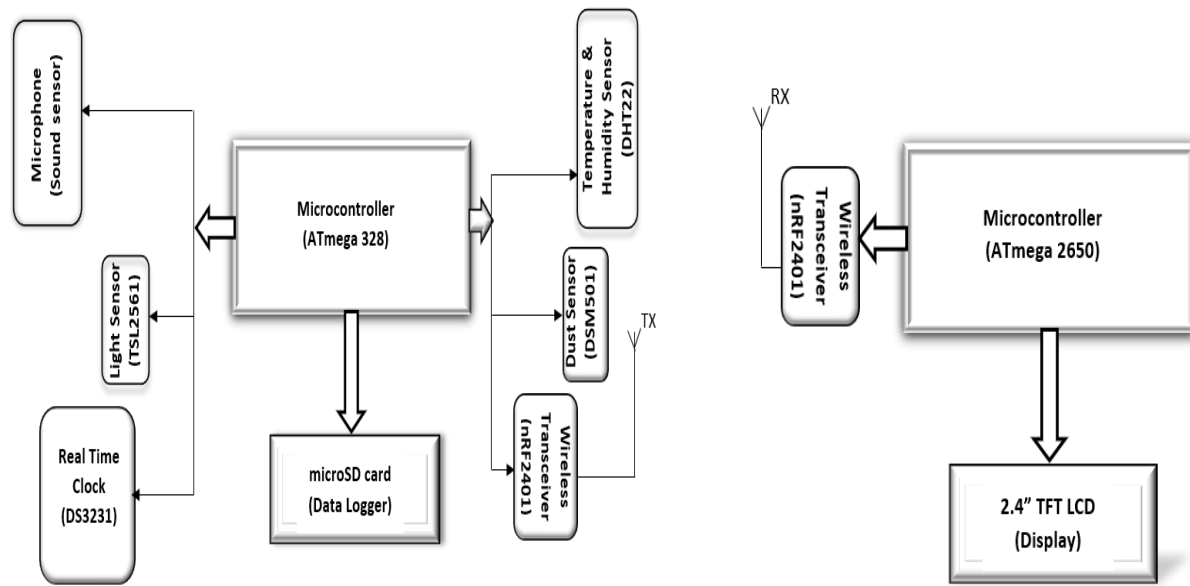
Figure 1: Schematic diagram of the developed EC-DAQS (a) Transmitter and (b) Receiver
