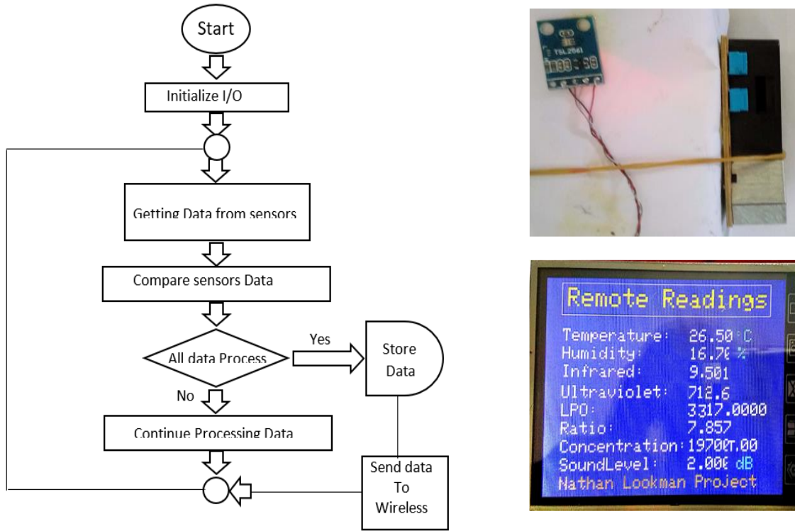
Figure 2: (a) Flow Chart of the EC-DAQS, (b) EC-DAQS Transmitter, (c) EC-DAQS Receiver display
