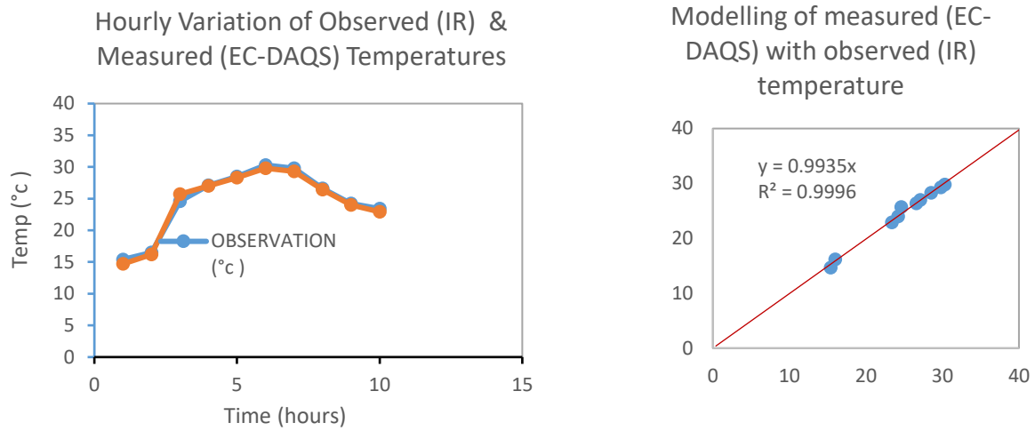
Figure 5: a) Comparison of observed (IR) and measured (DAQS) Temperatures b) Linear relationship between observed (IR) and measured (DAQS) readings
