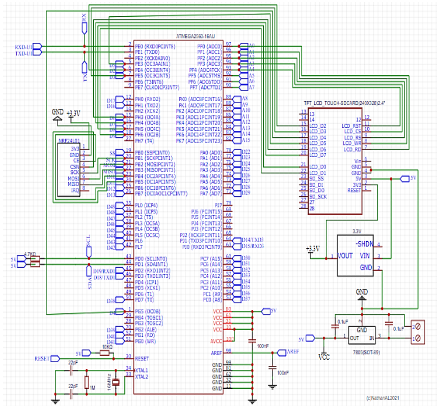
Figure 3: The Pin-Configuration of the developed EC-DAQS (a) Transmitter, (b) Receiver
