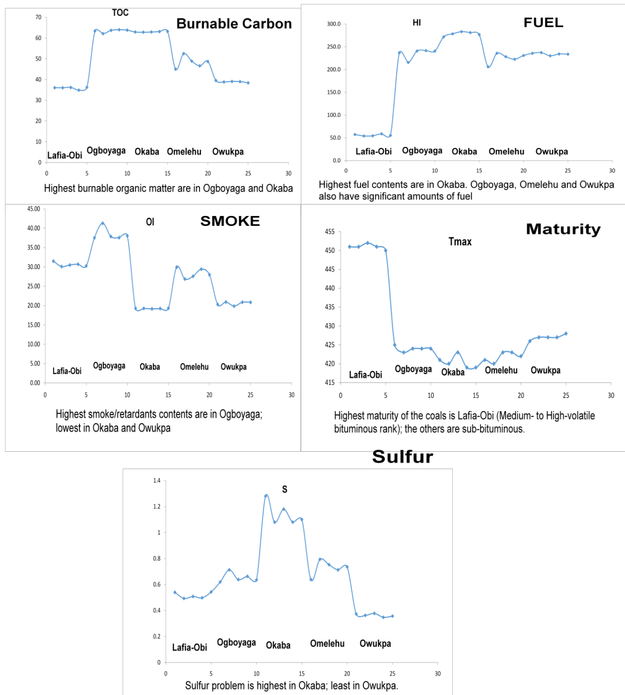
Fig. 10. Interpretation of Rock-Eval pyrolysis data shows that the Okaba coal deposit with the highest burnable organic matter, highest inherent fuel and least amounts of smoke is most suitable for smokeless coal fuel production and electricity generation in its present form. However, sulfur content presents some problems. The Ogbayaga and Omelehu coals will need defusinization.
