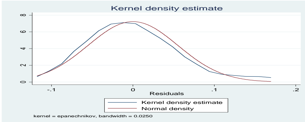
Figure 1: Testing the normality
