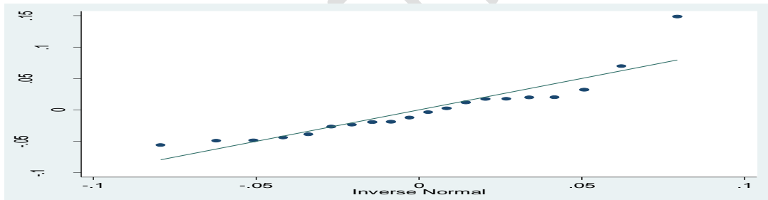
Figure 2 Testing for linearity (q-q plot)
