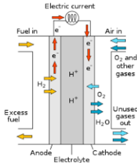
Fig 4 hydrogen fuel cell
