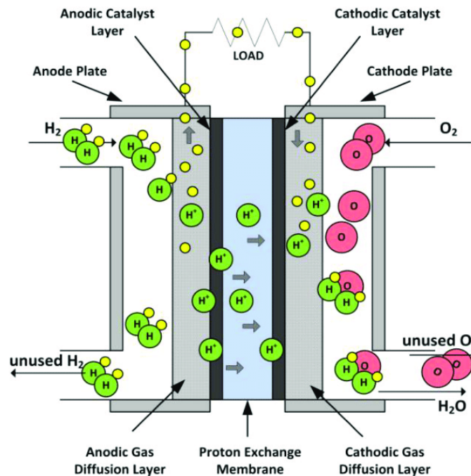
Fig 5 proton exchange membrane fuel cell
