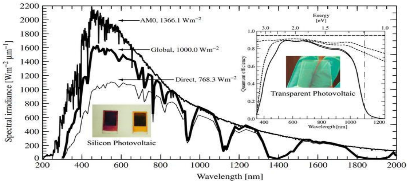
Fig 3 spectrum of light energy absorbed by transparent and silicon based cell
