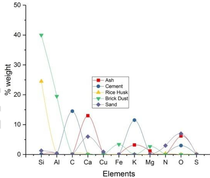
Fig.2. Elemental composition of the dust samples
