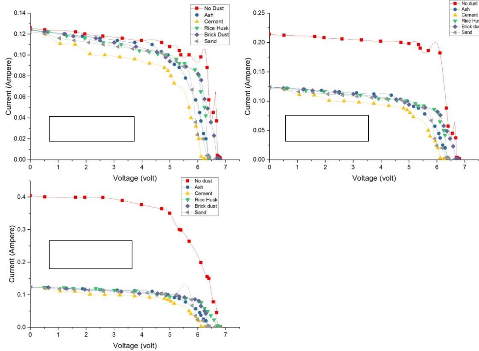
Fig.3. I - V characteristics for three different solar irradiances
