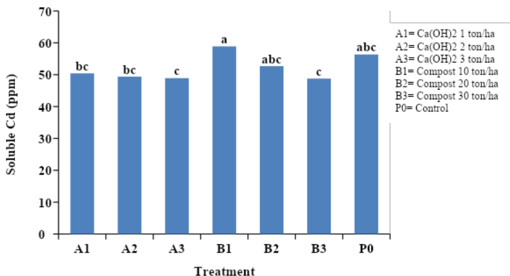
Figure 6. Effect of Ca(OH) 2 and compost on Cd
