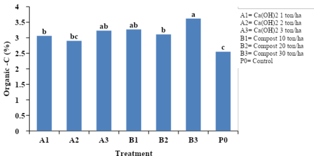
Figure 4. Effect of \text{Ca}(\text{OH})_2 and compost on soil organic C.
