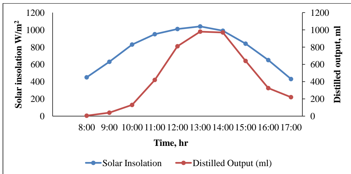
Fig.6. Hourly variation of the distilled output and solar insolation on 1 st April 2021
