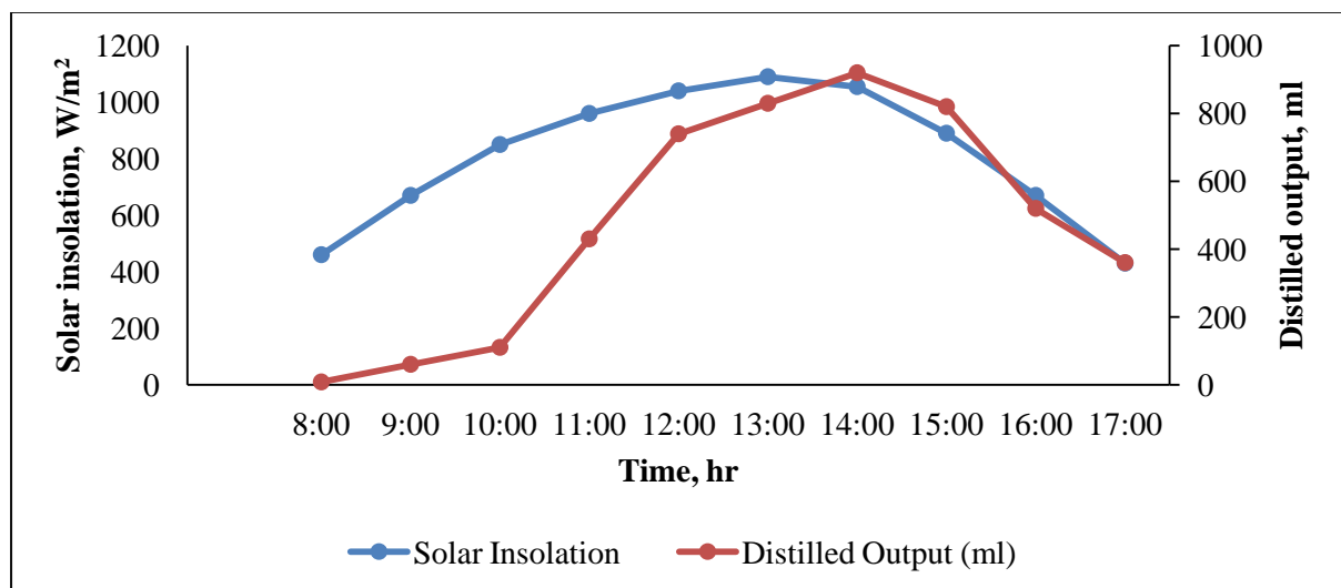
Fig.7. Hourly variation of the distilled output and solar insolation on 5 th April 2021
