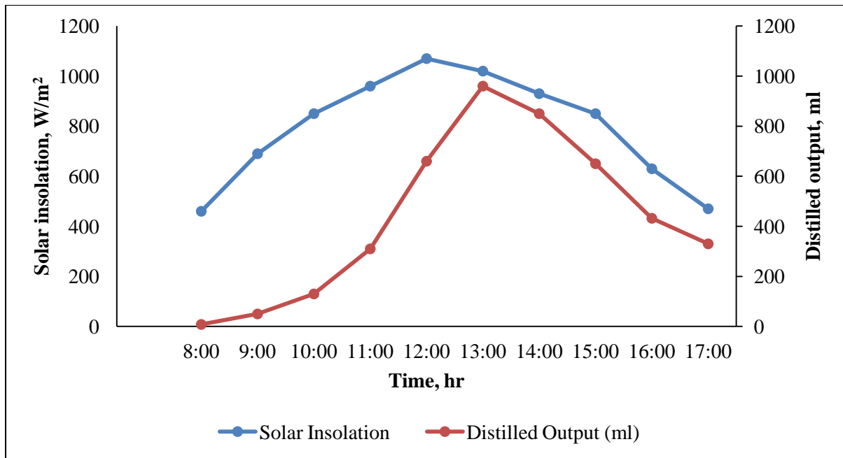
Fig.8. Hourly variation of the distilled output and solar insolation on 6 th April 2021
