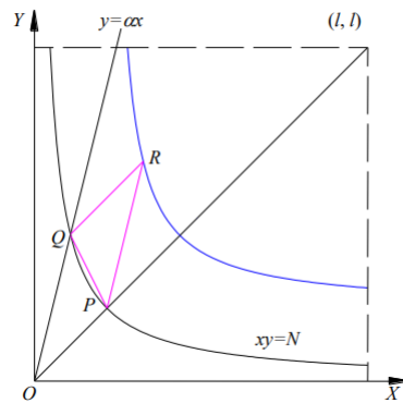
Figure 7: Hyperbola H:xy = N and locus of R
