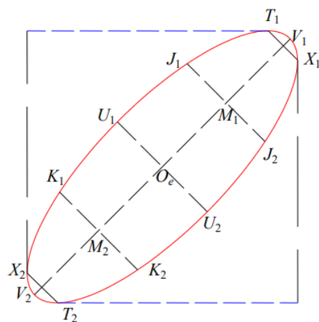
Figure 4: Points on ellipse \Gamma_e
