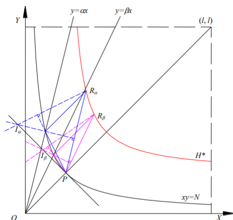
Figure 9: Orthocenters concurrent with tangent line at P
