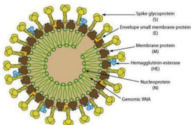
Figure 1. structure of SARS-COV-2 [5]
