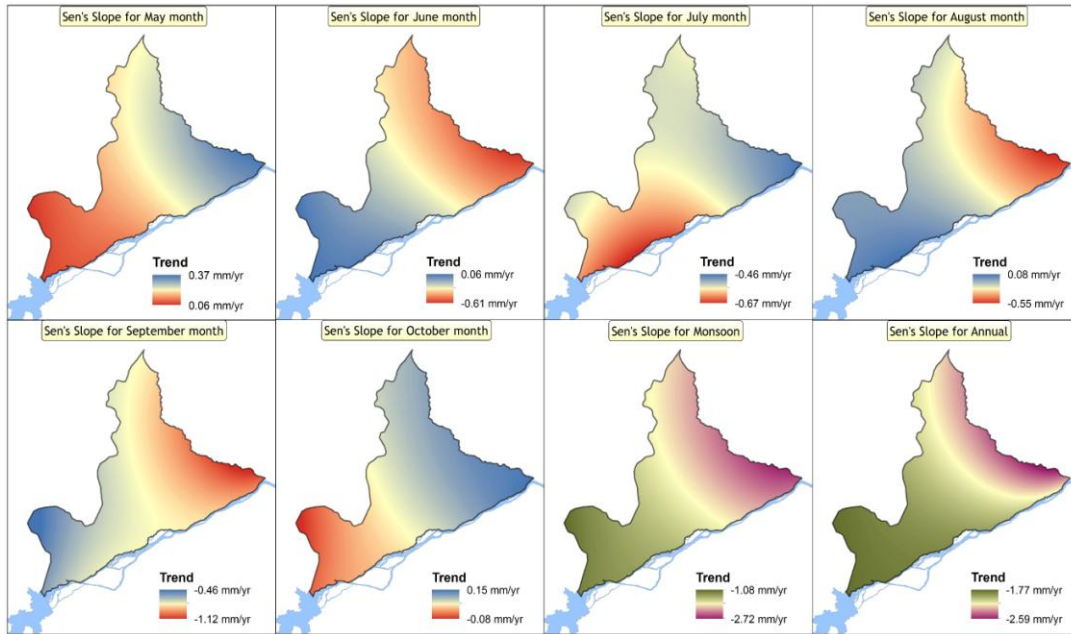
Figure 7: Spatio – Temporal distribution of trend in Rainfall Pattern over NLBC command by MK Test.
