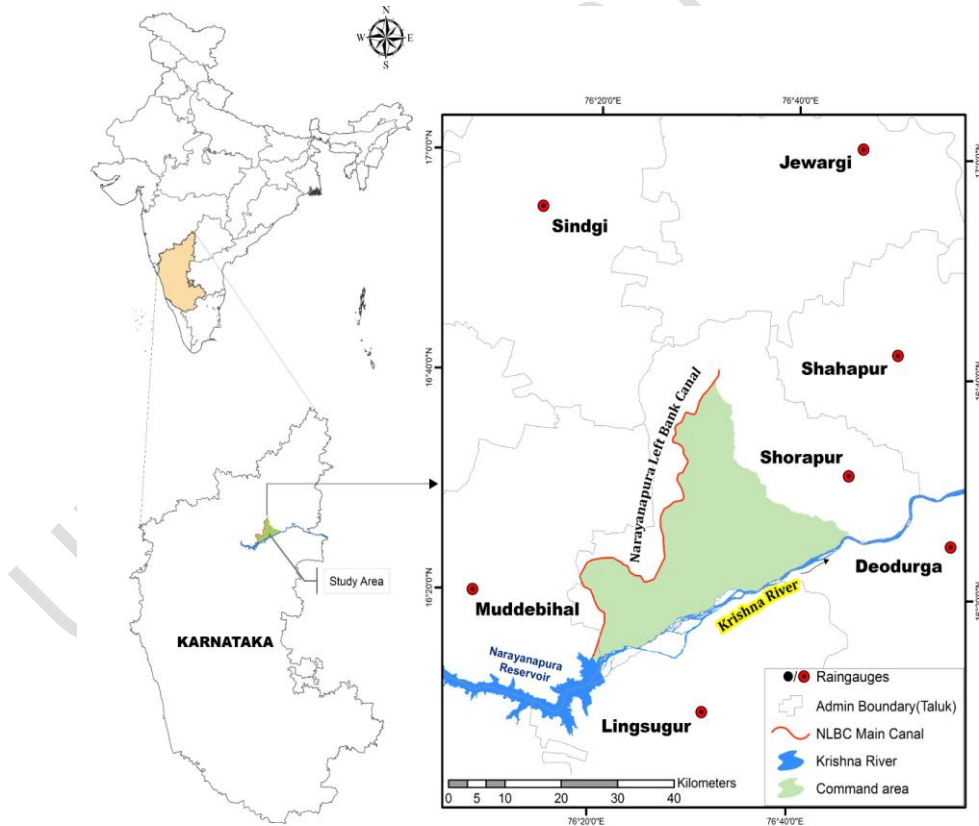
Figure 1: Study area map with influencing rain gauges.
