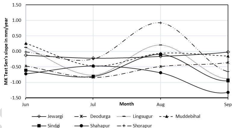
Figure 8: Sen's Slope variations of Raingauges for Monsoon months.
