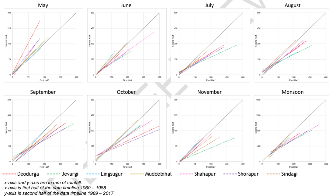
Figure 9: ITA trendline graphs representation for monthly and monsoon rainfall.
