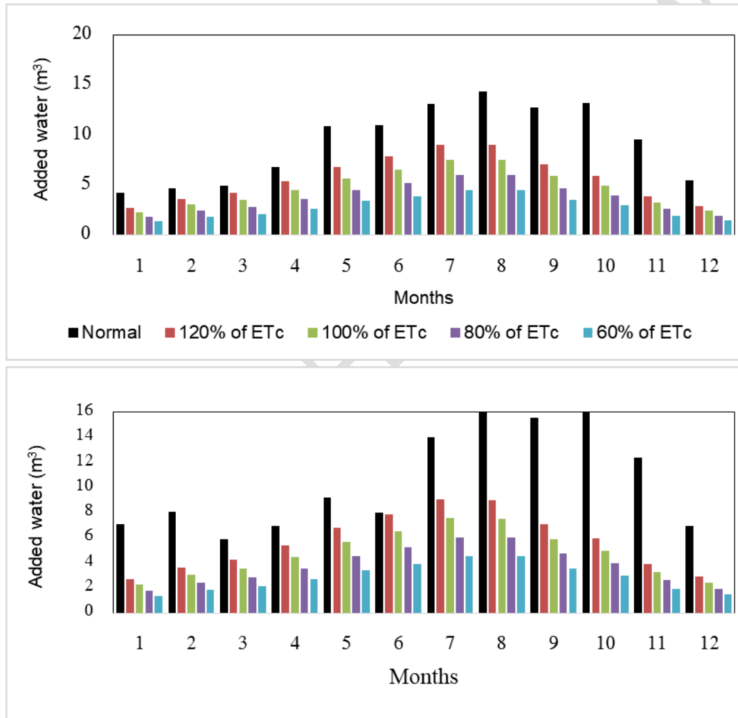
Fig. 1. Comparison between traditional and different deficit irrigation on WR ( m^3/month ). A: well water and B; treated water
