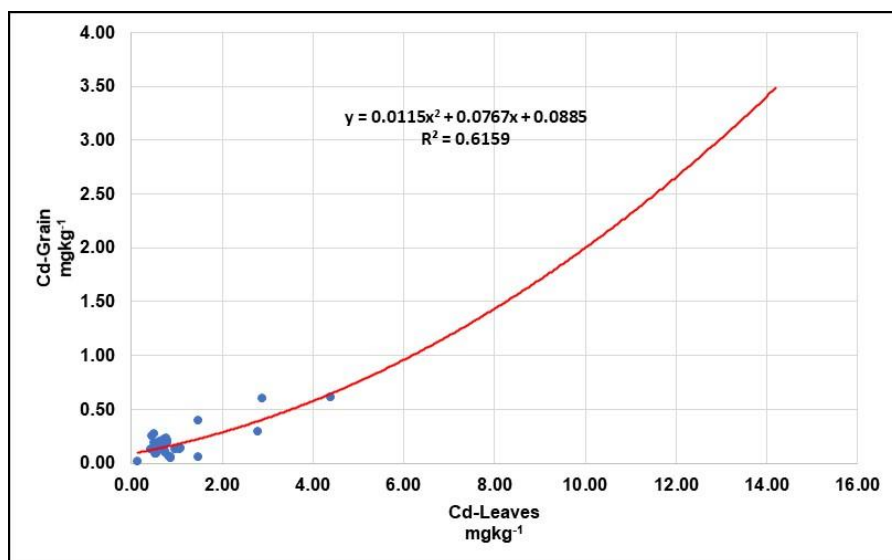
Fig. 14. Forecast of the behavior of the translocation of Cd in leaves and Cd in grains, according to sampling in 16 sites and doses of Cd applied to the soil in Creole cocoa genotype AS-CP 26-61 (mulatto).
