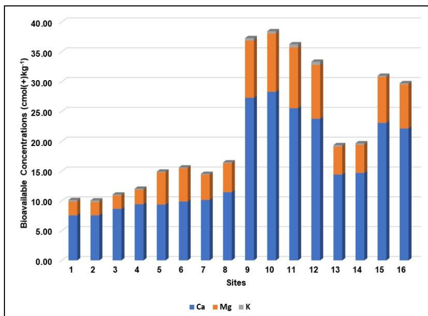
Fig. 5. Average Ca-Mg-K concentrations in soils, Almirante – Bocas del Toro, Republic of Panama.
