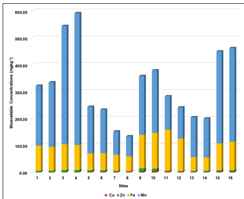
Fig. 6. Average concentrations of Cu-Zn-Fe-Mn in soils, Almirante – Bocas del Toro, Republic of Panama.
