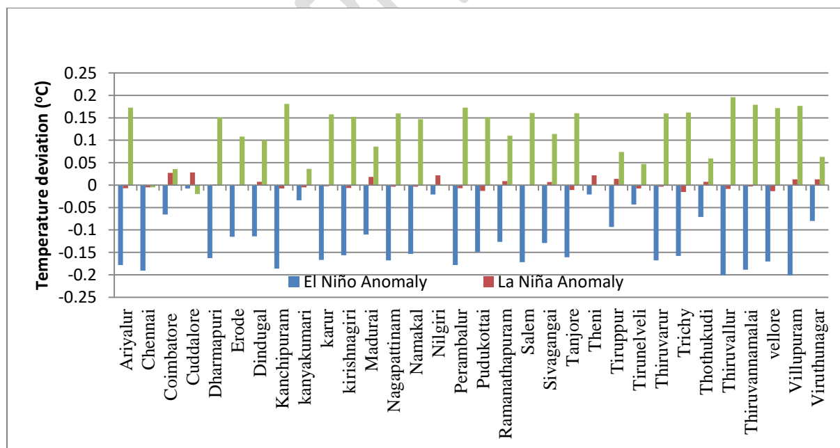
Fig. 3. Influence of ENSO on Hot Weather Period (HWP) mean maximum temperature over different districts in Tamil Nadu (1971 - 2013)
