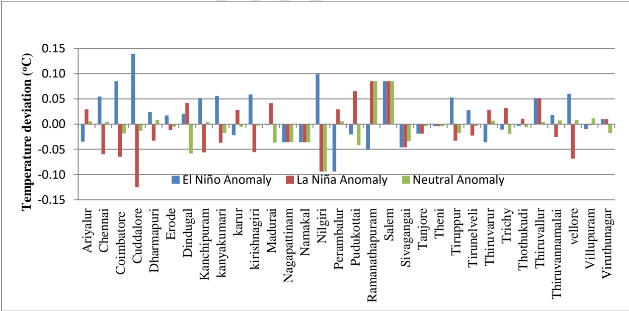
Fig.7. Influence of ENSO on NEM mean maximum temperature over different districts in Tamil Nadu (1971 - 2013)
