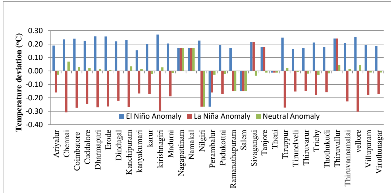
Fig.8. Influence of ENSO on NEM mean minimum temperature over different districts in Tamil Nadu (1971 - 2013)
