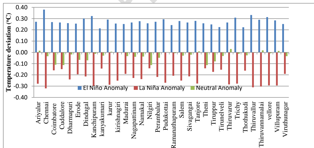
Fig.5. Influence of ENSO on SWM mean maximum temperature over different districts in Tamil Nadu (1971 - 2013)
