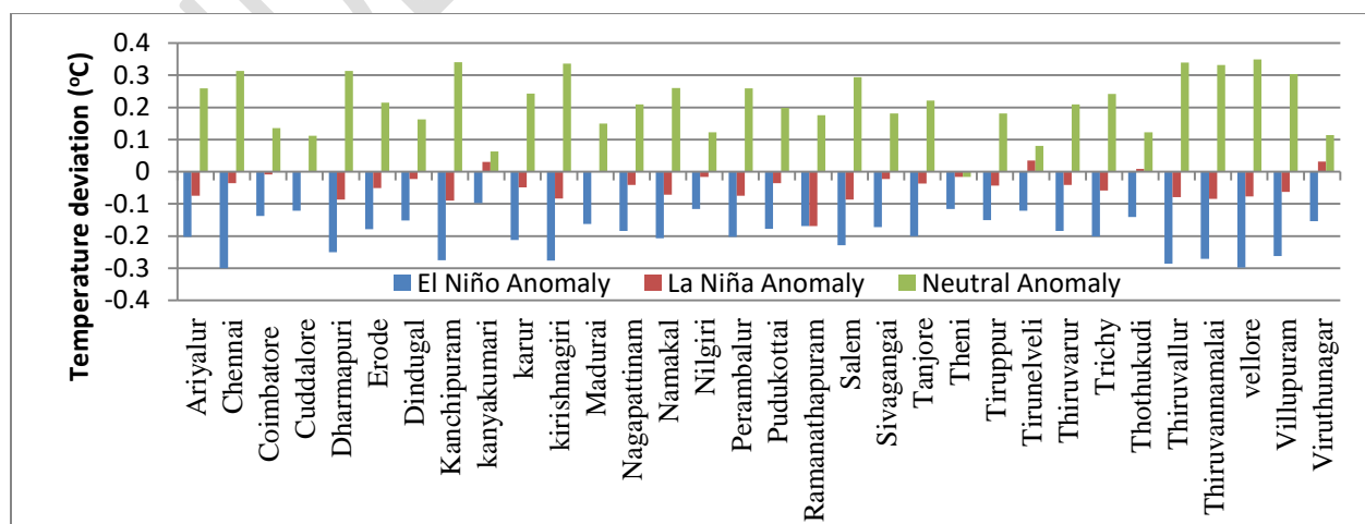
Fig.1. Influence of ENSO on Cold Weather Period (CWP) mean maximum temperature over different districts in Tamil Nadu (1971 - 2013)
