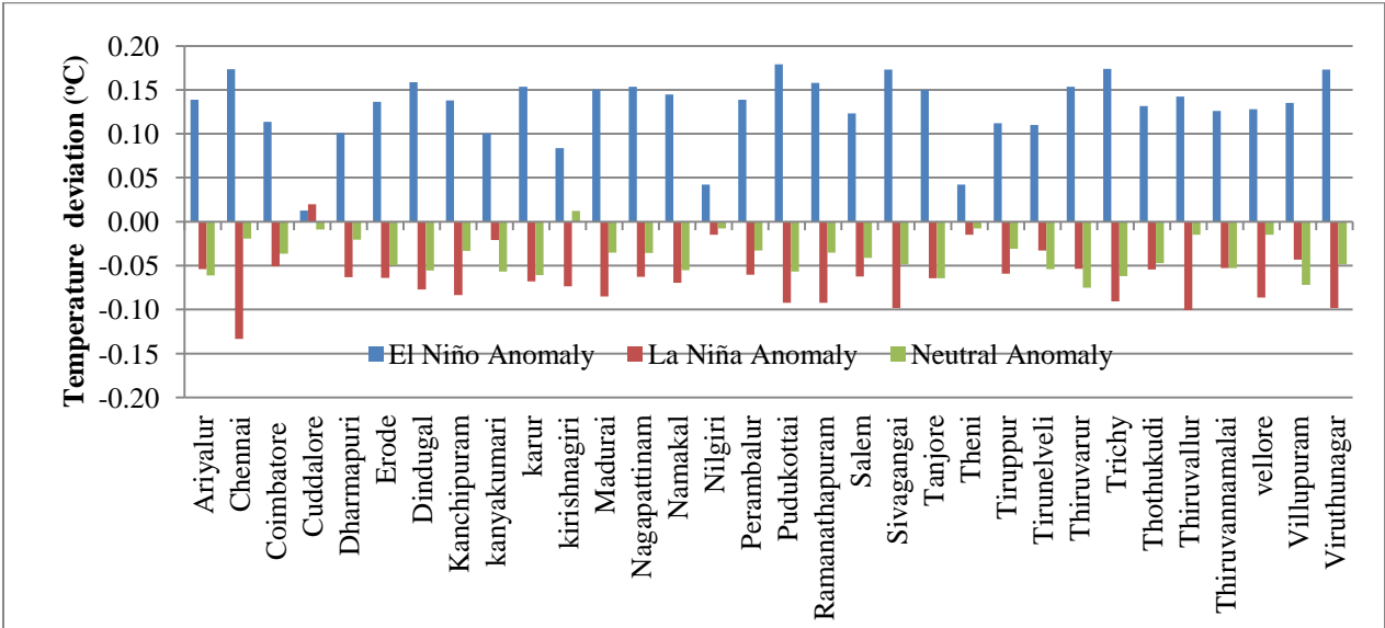
Fig.6. Influence of ENSO on SWM mean minimum temperature over different districts in Tamil Nadu (1971 - 2013)
