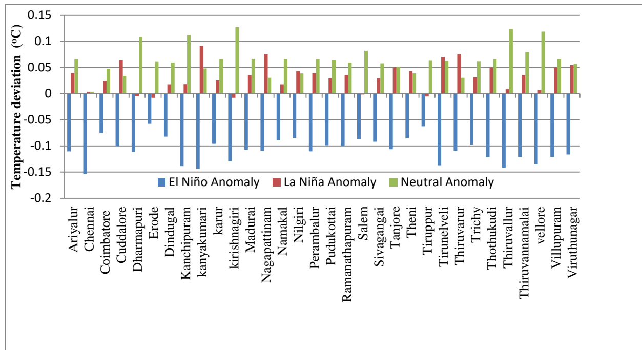
Fig.4. Influence of ENSO on Hot Weather Period (HWP) mean minimum temperature over different districts in Tamil Nadu (1971 - 2013)
