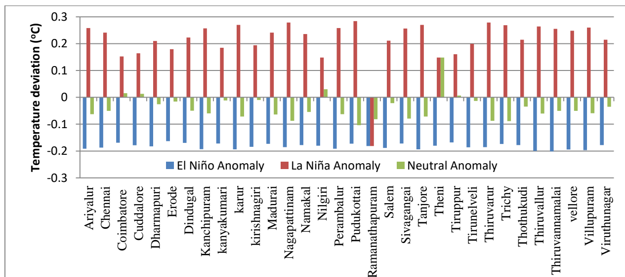
Fig.2. Influence of ENSO on Cold Weather Period (CWP) mean minimum temperature in different districts in Tamil Nadu (1971 - 2013)
