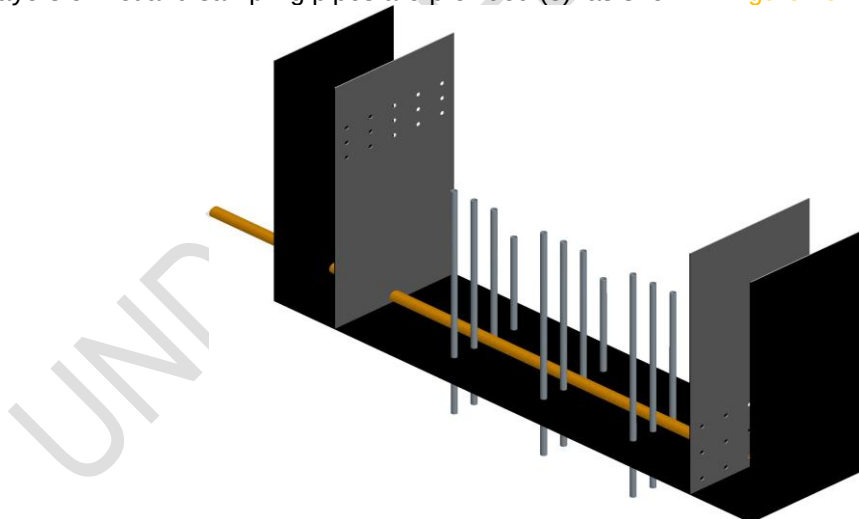
Fig. 10. Digital isometric view of the different sampling points to collect samples from different layers in laboratory scale constructed wetland system
