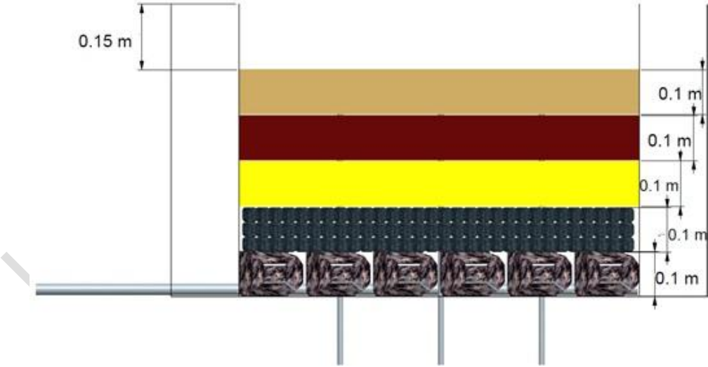
Fig. 5. Thickness of the each layer in laboratory scale constructed wetland system
