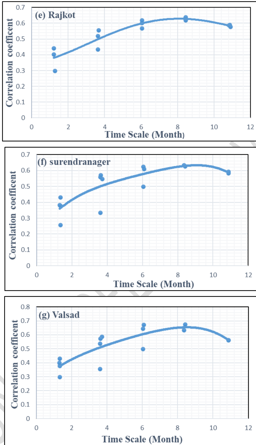
Fig. 3 Average correlation of a particular time-step drought index with all other indices time scales at (a) Ahmedabad, (b) Bharuch, (c) Jamanager, (d) Kutch, (e) Rajkot, (f) Surendranagar, and (g) Valsad Districts.
