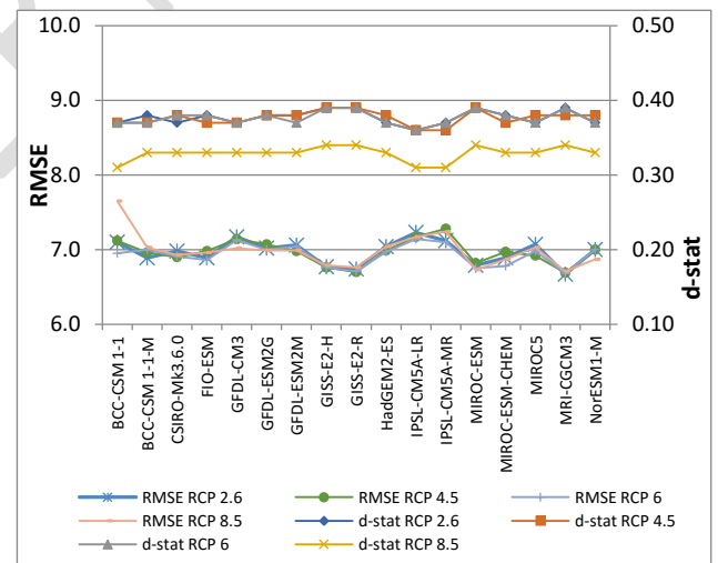
Fig. 1(d): Monthly accumulated Solar radiation ( \text{MJ m}^{-2} \text{month}^{-1} )
