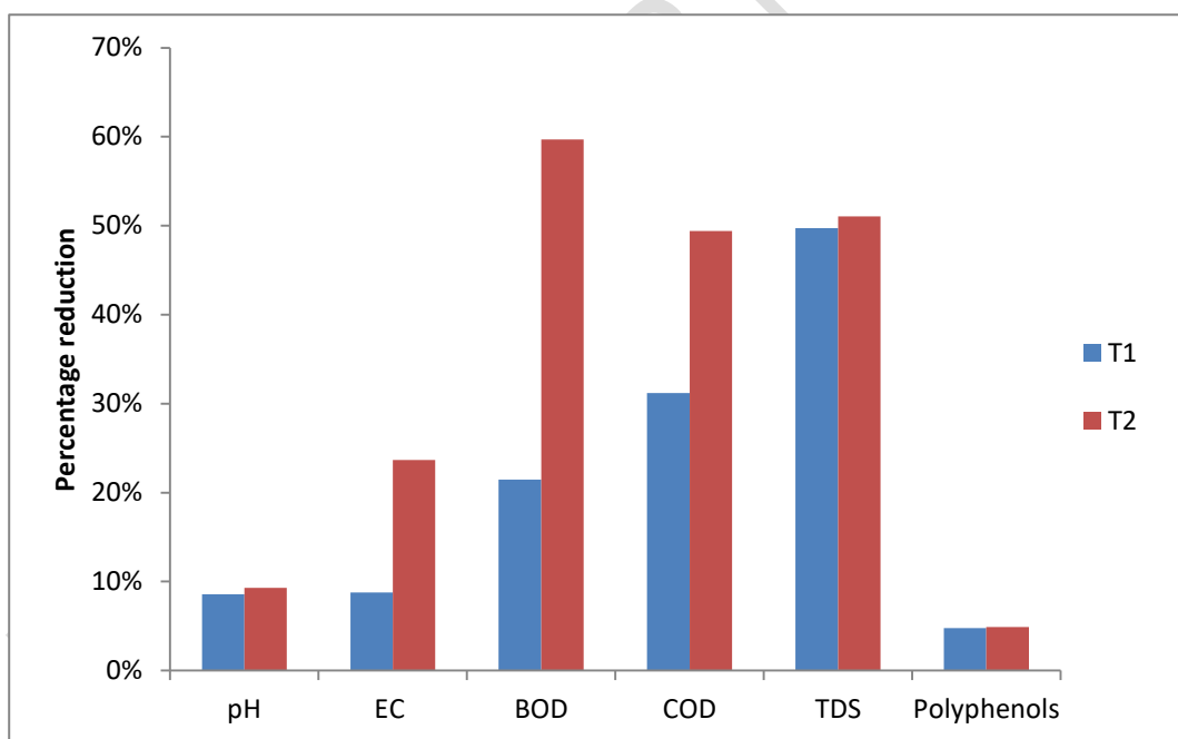
Fig. 3 Percentage reduction of Physio-chemical characters
