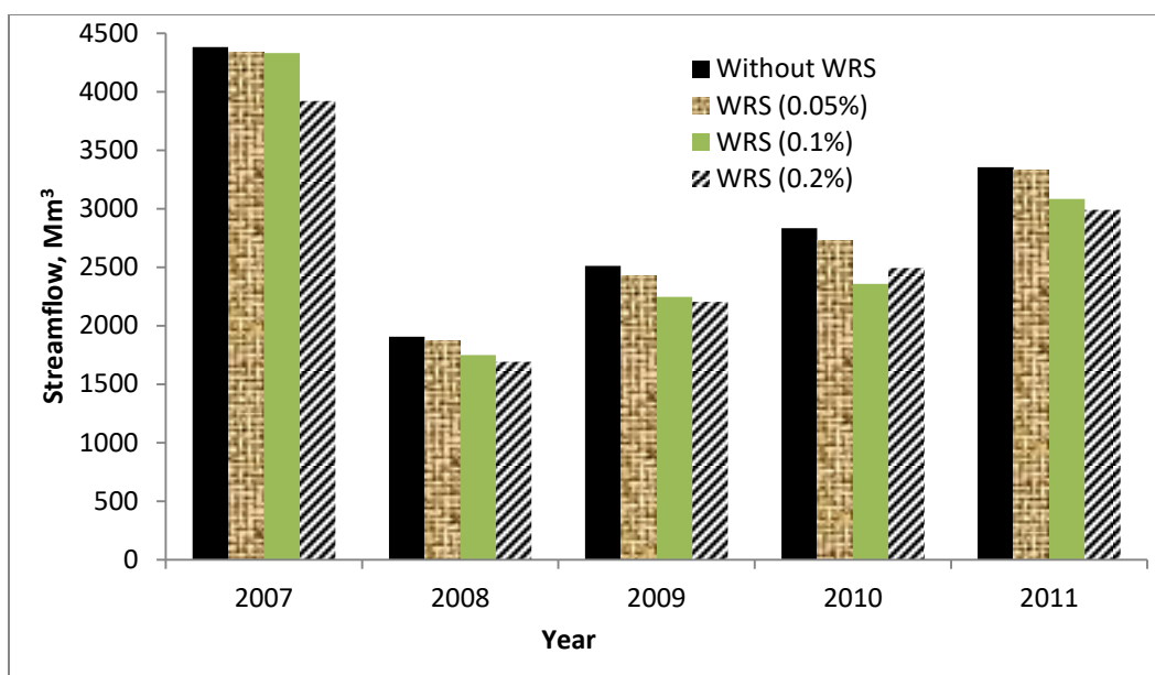
Fig. 5. Annual streamflow under different levels of WRS
