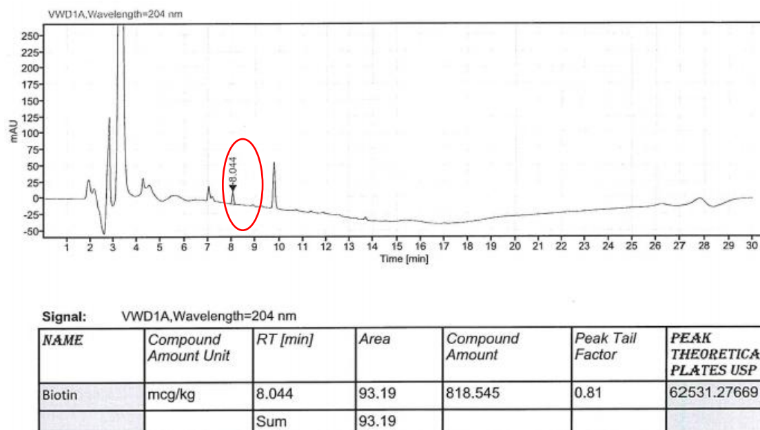
Figure 1: HPLC chromatogram with biotin peak eluted at 8.044min
