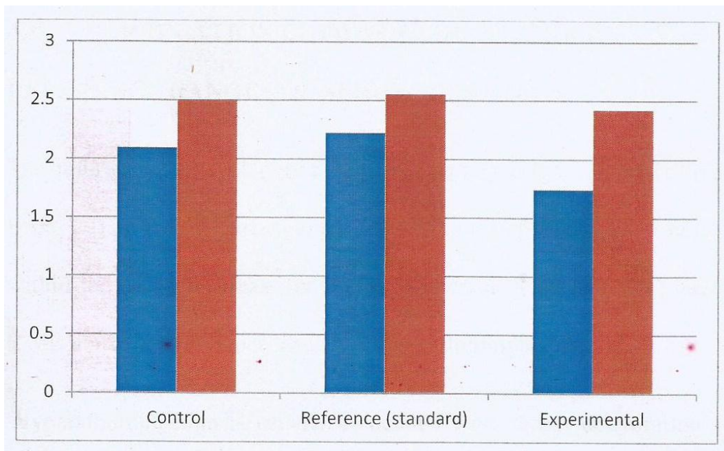
Figure 1: Serum calcium representation of both experimental, control and reference (standard) showing the minimum and maximum points for each.
