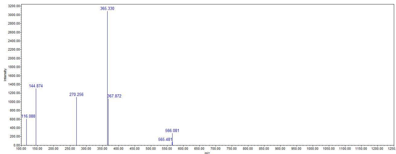
Fig 6 Mass spectrum for Acetylaustrinide ( Diterpenoid) identified in M.p leaf (RT 6.77)
