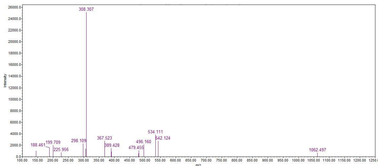
Figure 3: Dihydrocapsaicin (Meltosyphenol) identified in M.p seed ( RT 12.66)
