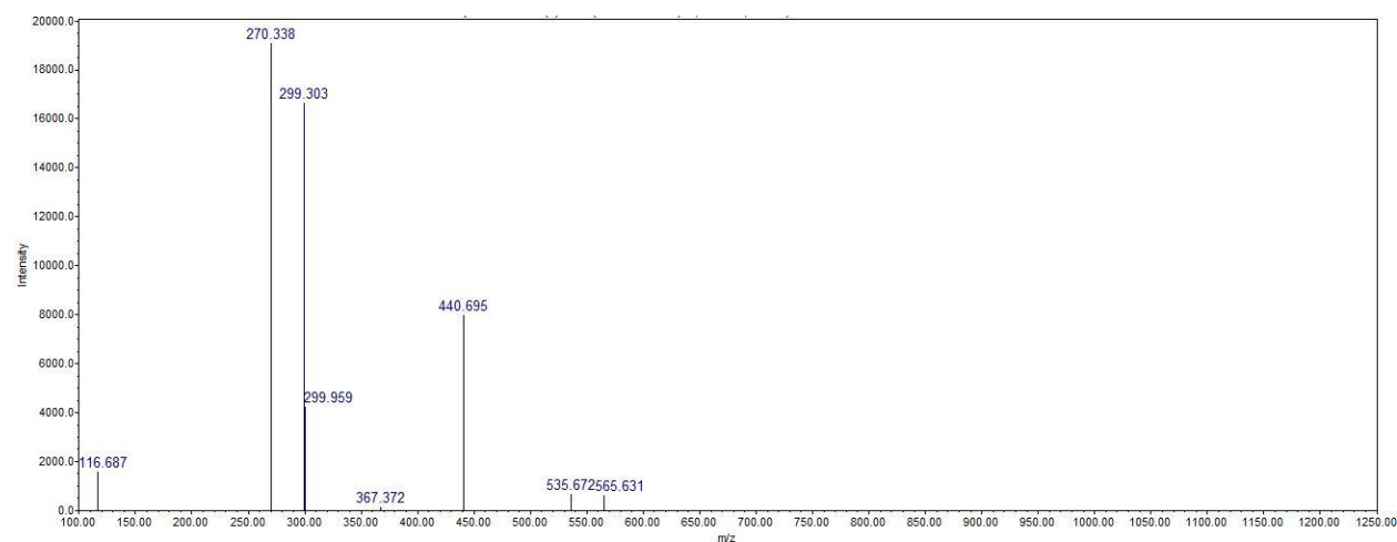
Fig 5 Mass spectrum for Epioxylubianin (Sesqueneperoxide) ) identified in M.p leaf (RT 10.52)
