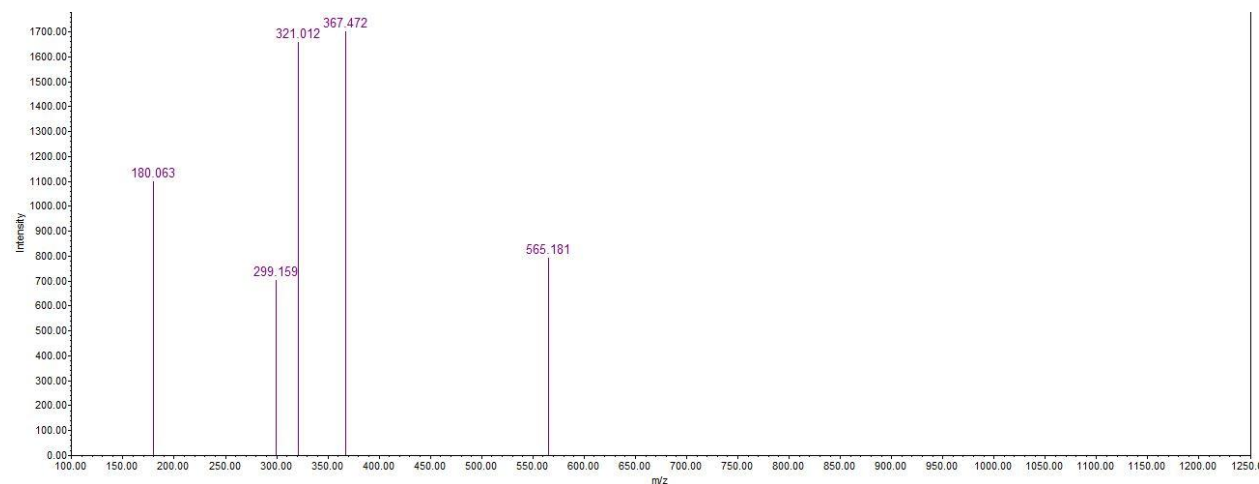
Fig 7 furocoumaric acid glycoside (phenolic glycoside) identified in M.p leaf (RT 6.02)
