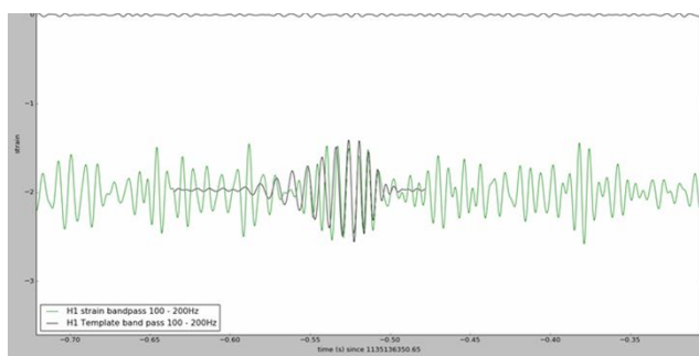
Fig.3 About 0.50 seconds before LIGO's so-called gravitational wave burst , the noise waveform (green curve) appeared in Hanford interferometer and the theoretical and filtered waveform (black curve).
