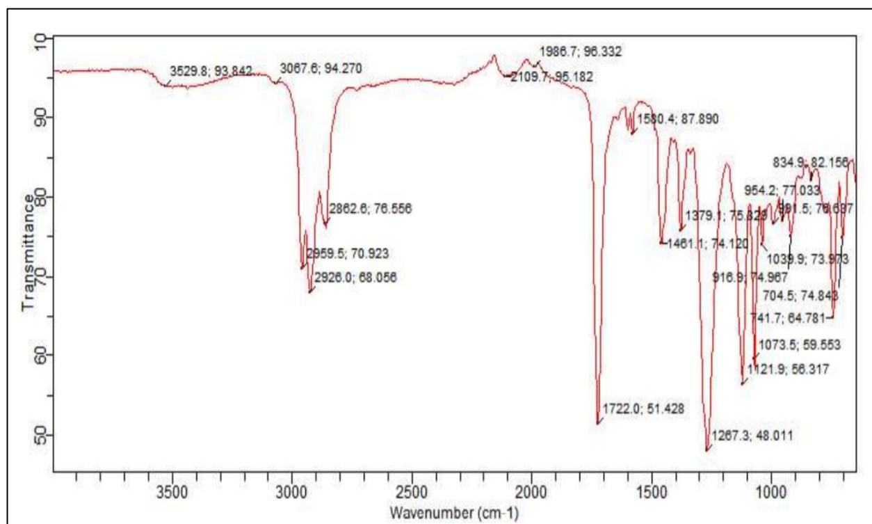
Figure 3: FTIR spectra of Citrus aurantium var. amara essential oil ranging from wavenumbers 4,000-650 cm -1 as versus transmittance.
