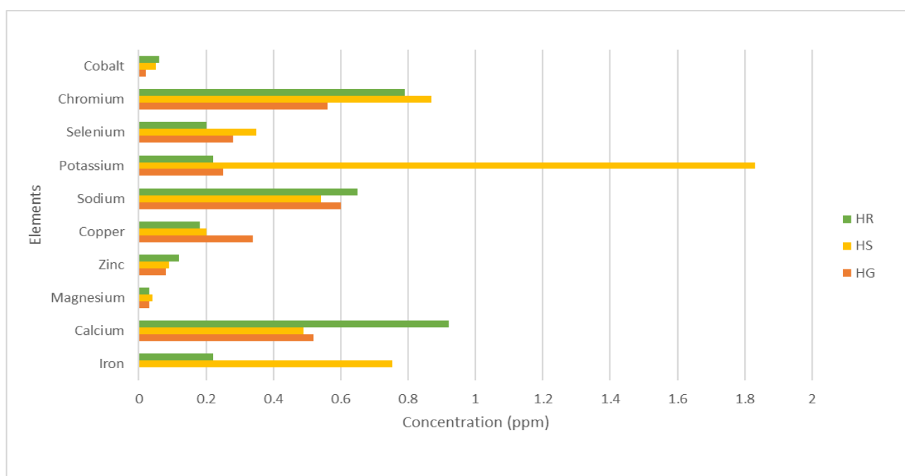
Figure 1: Analysis of elemental composition of HR, HG, HS. HR- Hibiscus acetosolla Welw, HG- Hibiscus cannabinus L, HS- Hibiscus sabdariffa L,
