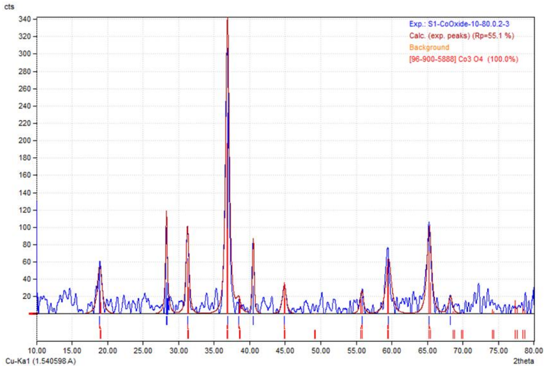
Fig (1). XRD Diffraction Pattern Graphic of Co 3 O 4
