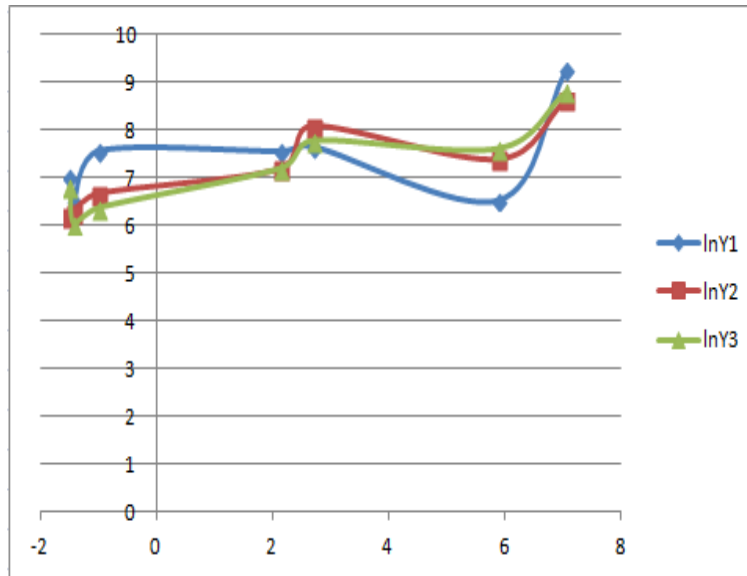
Fig. 5. ln(Energy) Versus ln(Viscosity).
