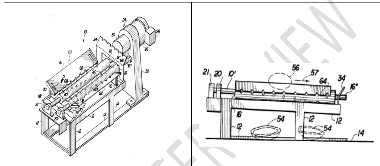
Fig. 1.1 Twin roller coconut dehusking machine
