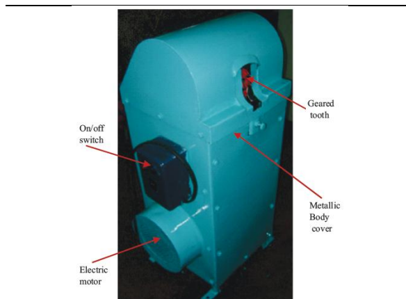
Fig. 2.5 ICAR-CPCRI power operated coconut de-shelling machine
