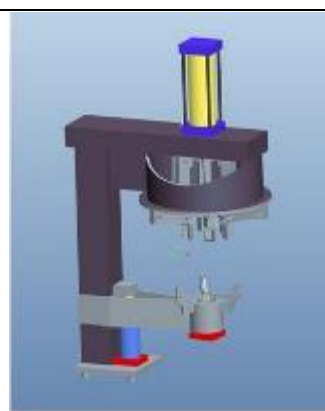
Fig. 1.6 Hydraulic coconut dehusking machine.
