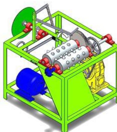
Fig. 1.11 Automated coconut dehusking and crown removal machine
