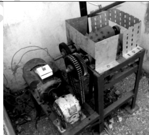
Fig. 1.19 Spiked and rollers type coconut dehusking machine
