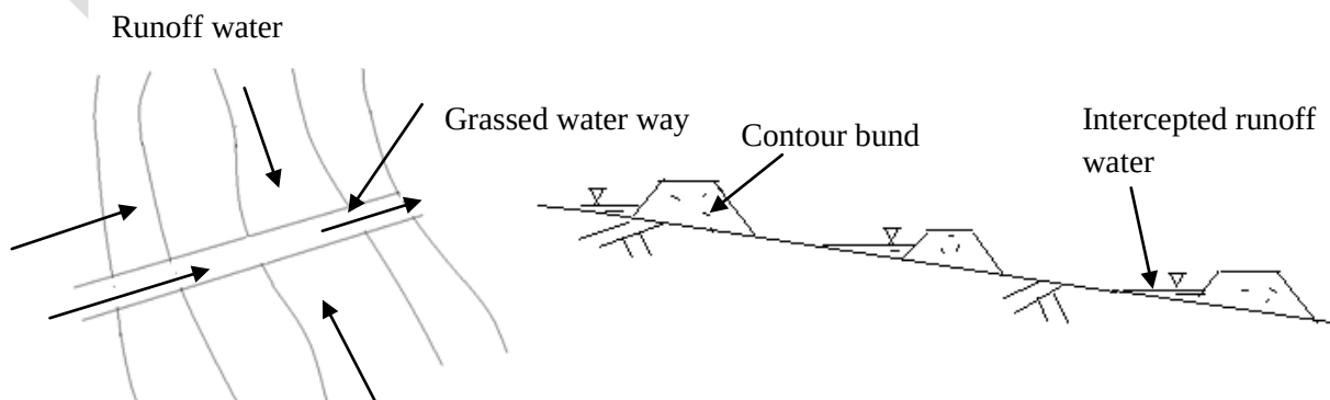
Fig.3 Contour bunds and grassed disposal channel
