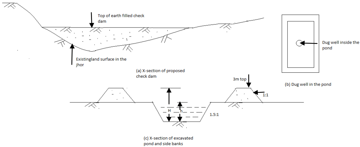
Fig.2 Check dam, ponds and dug-well sections and locations
