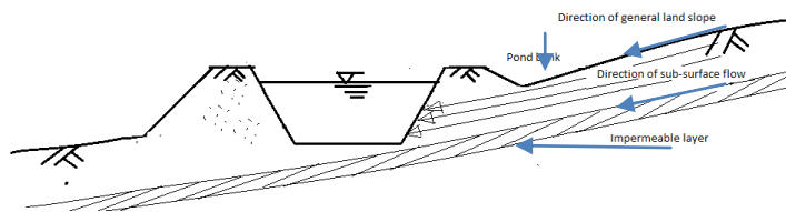
Fig.12 Pond with sub-surface flow in it
