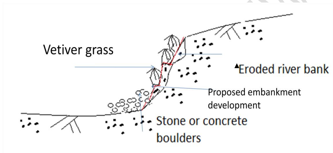
Fig.5 River bank erosion control measures
