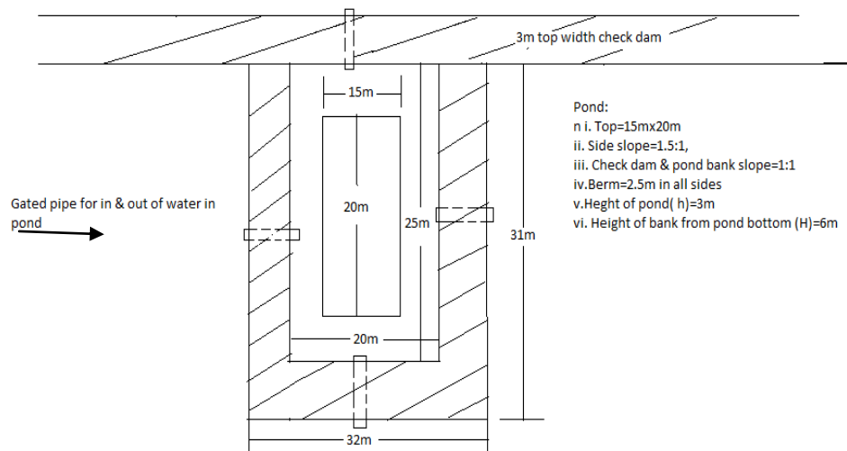
Fig.1 Schematic diagram of proposed water course in Jhor
