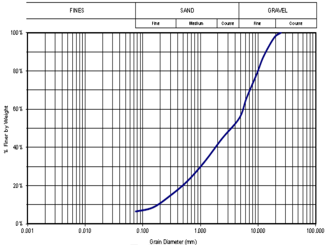
Fig. 2: Particle Size Distribution Curve
