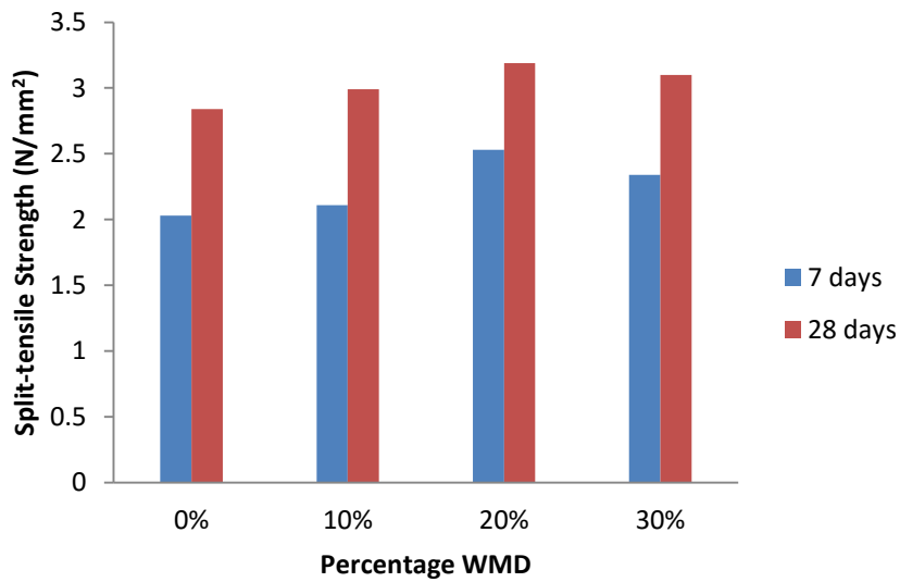
Fig. 5: Graph showing results of split-tensile strength test
