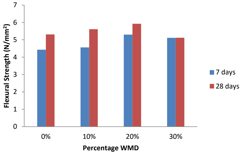
Fig. 6: Graph showing results of flexural strength test
