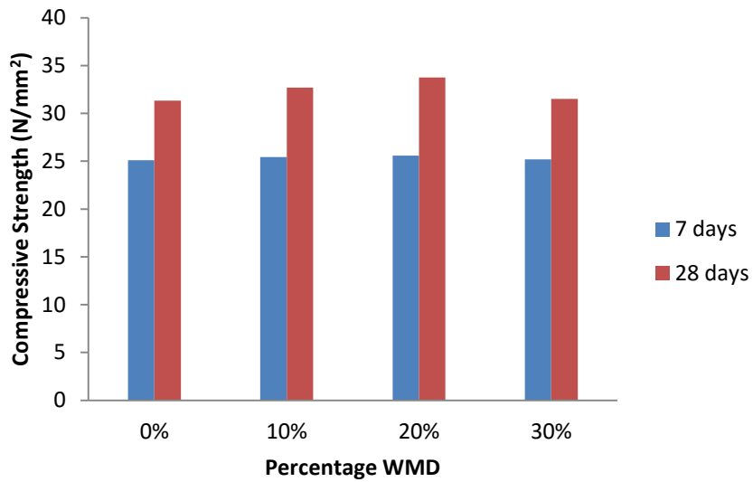
Fig. 4: Graph showing results of compressive strength test
