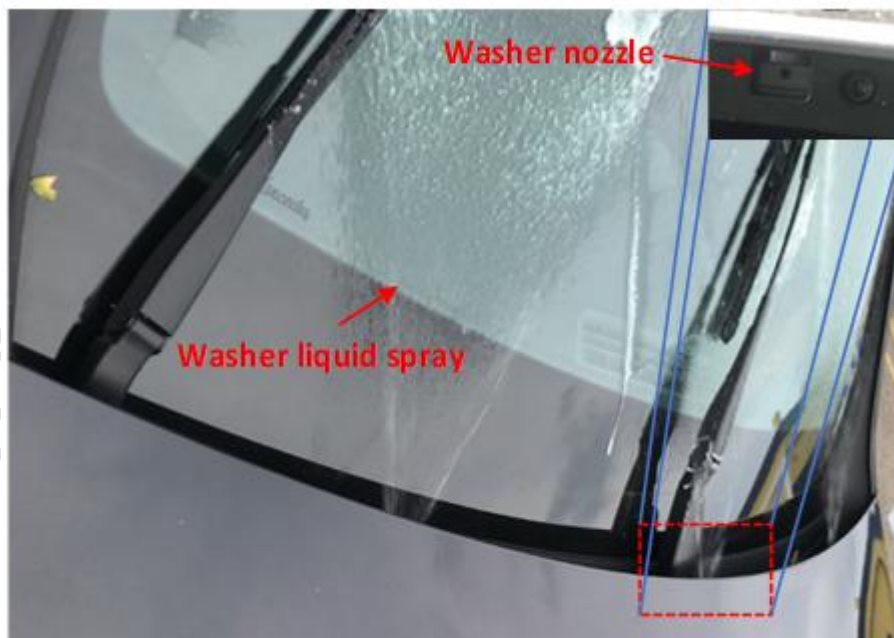
Fig. 26. Spraying of washer liquid
