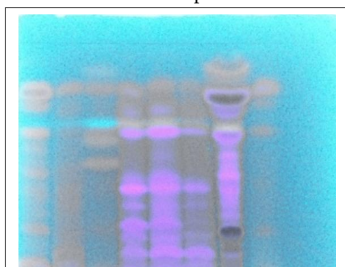
Figure 9. Chromatogram for alkaloids [Mobile phase: Toluene/ethyl acetate/diethylamine (35: 10: 5); Detection: \text{NaNO}_2 5%]. Alkaloids are characterized by the presence of orange spots.
