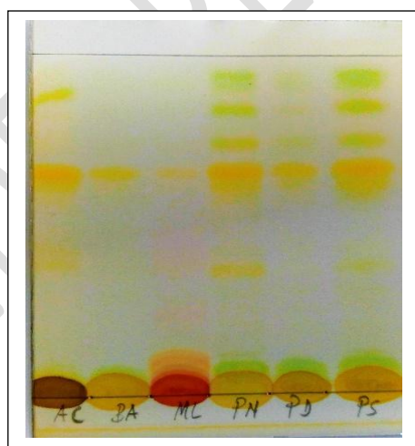
Figure 9. Chromatogram for alkaloids [Mobile phase: Toluene/ethyl acetate/diethylamine (35: 10: 5); Detection: \text{NaNO}_2 5%]. Alkaloids are characterized by the presence of orange spots.
