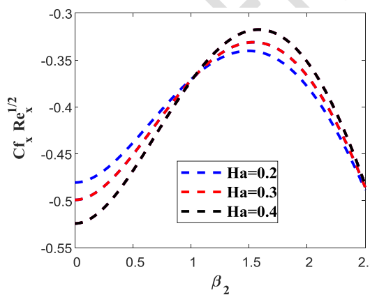
Fig.22. Effects of Hartman and Deborah numbers
