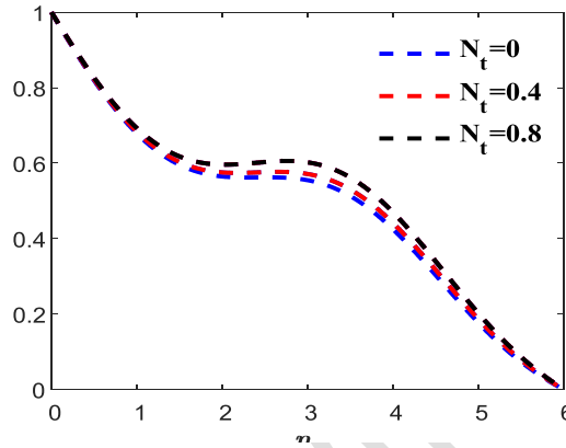
Fig.9 Effect of thermophoresis
