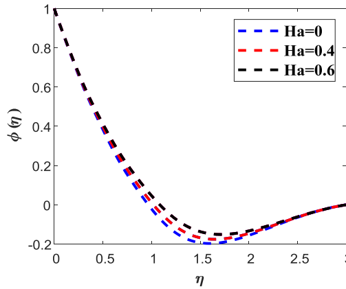
Fig.20. Effect of Hartman number
