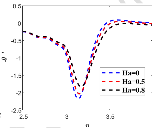
Fig.27. Effect of Hartman number
