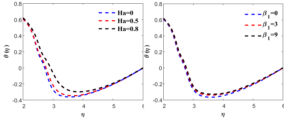
Fig.12. Effect of Hartman number Fig.13. Effect of relaxation-retardation
