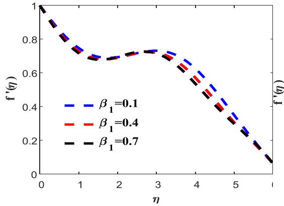
Fig.8. Effect of relaxation-retardation
