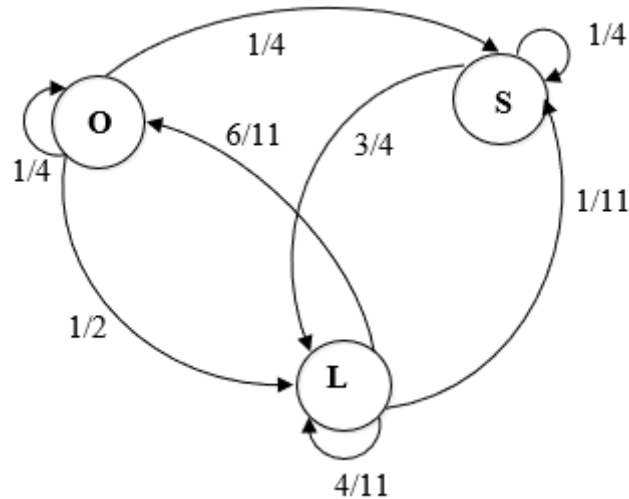
Markov Transitional Matrix for College of Humanities and Legal Studies (CHLS)
