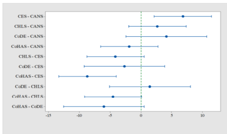
Figure 3: Fisher Pairwise Comparisons for the Colleges
