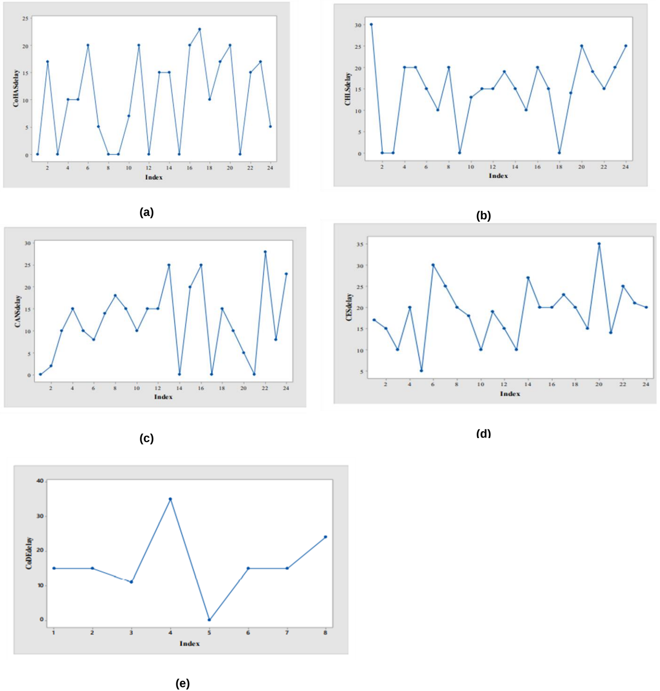
Figure 2: Time Series Plot Analysis of the pattern of delays in engagement schedules for the Colleges
